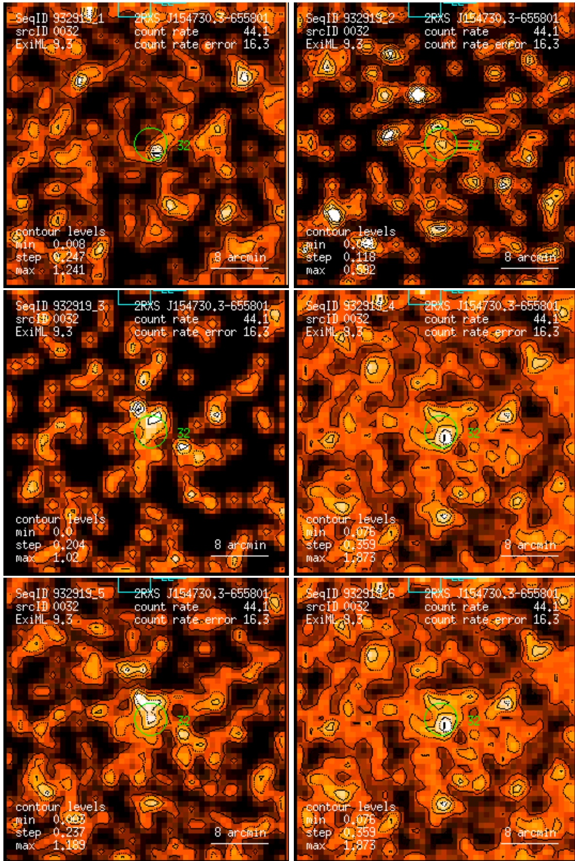
Figure 32: RASS 932919: detection 0032: band rate images, Gaussian filter: (1) PSPC channels 11 – 41, (2) 52 – 90, (3) 91 – 201, (4) 11 – 235, (5) 52 – 201, (6) 11 – 201. Broad band rates in counts/ks. Band rate contour levels in counts/ks/arcmin 2 .
