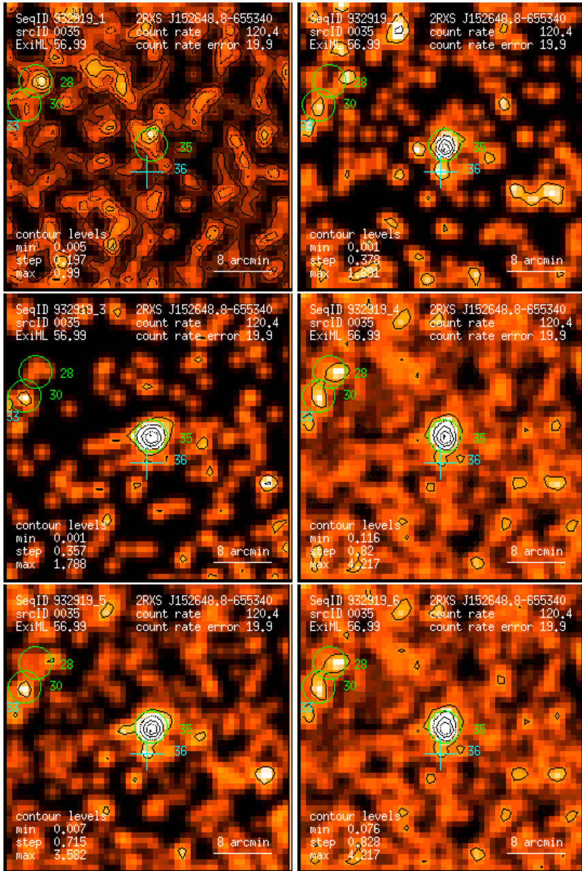
Figure 35: RASS 932919: detection 0035: band rate images, Gaussian filter: (1) PSPC channels 11 – 41, (2) 52 – 90, (3) 91 – 201, (4) 11 – 235, (5) 52 – 201, (6) 11 – 201. Broad band rates in counts/ks. Band rate contour levels in counts/ks/arcmin 2 .
