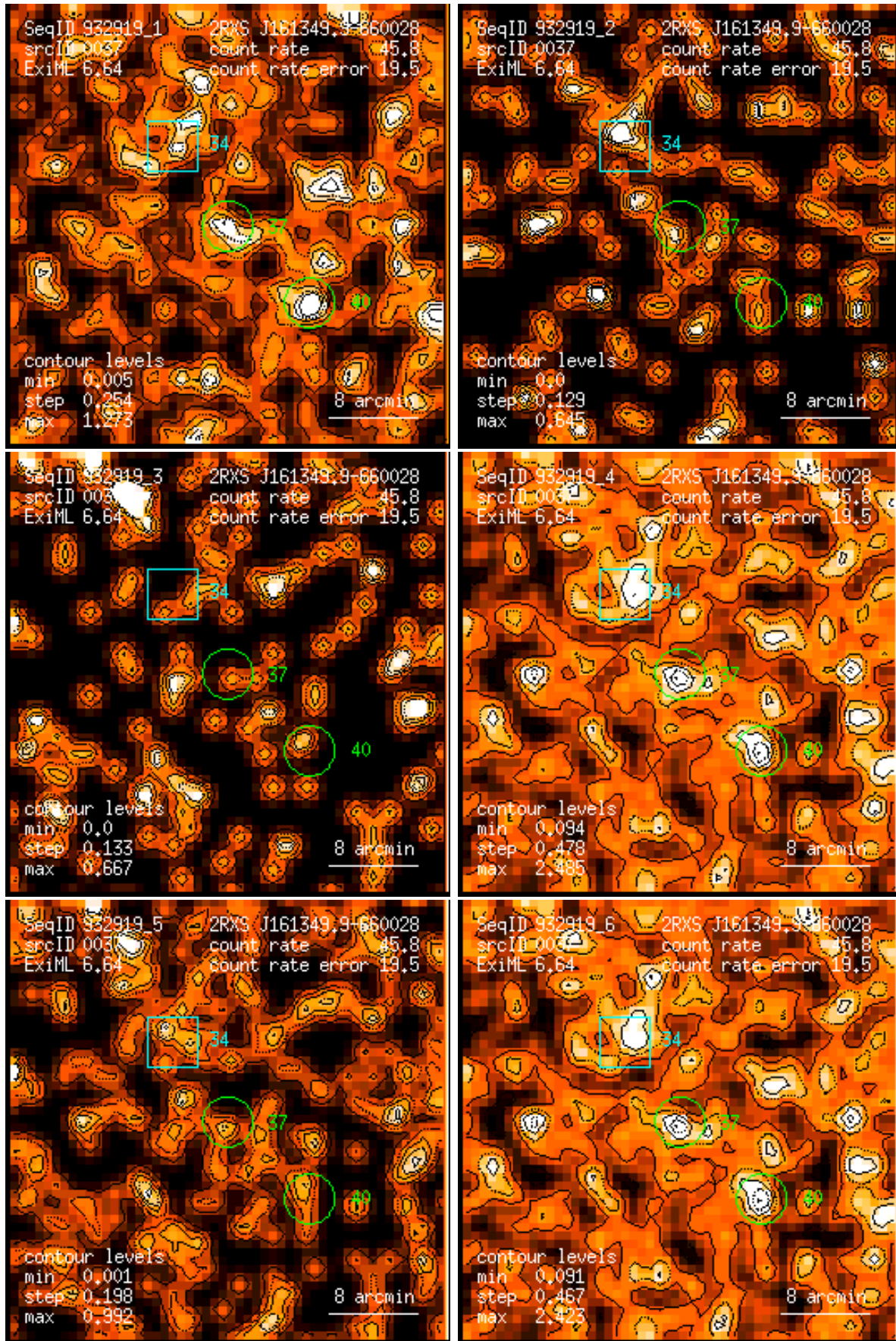
Figure 37: RASS 932919: detection 0037: band rate images, Gaussian filter: (1) PSPC channels 11 – 41, (2) 52 – 90, (3) 91 – 201, (4) 11 – 235, (5) 52 – 201, (6) 11 – 201. Broad band rates in counts/ks. Band rate contour levels in counts/ks/arcmin 2 .
