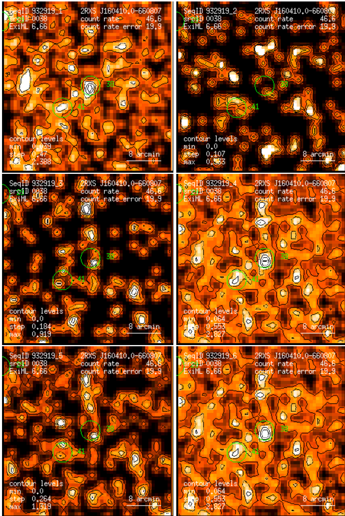
Figure 38: RASS 932919: detection 0038: band rate images, Gaussian filter: (1) PSPC channels 11 – 41, (2) 52 – 90, (3) 91 – 201, (4) 11 – 235, (5) 52 – 201, (6) 11 – 201. Broad band rates in counts/ks. Band rate contour levels in counts/ks/arcmin 2 .
