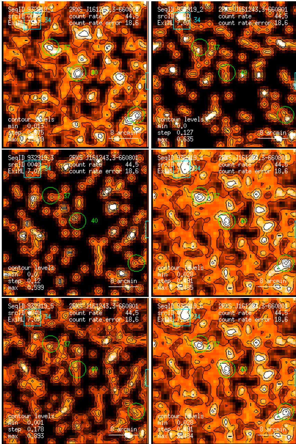
Figure 40: RASS 932919: detection 0040: band rate images, Gaussian filter: (1) PSPC channels 11 – 41, (2) 52 – 90, (3) 91 – 201, (4) 11 – 235, (5) 52 – 201, (6) 11 – 201. Broad band rates in counts/ks. Band rate contour levels in counts/ks/arcmin 2 .
