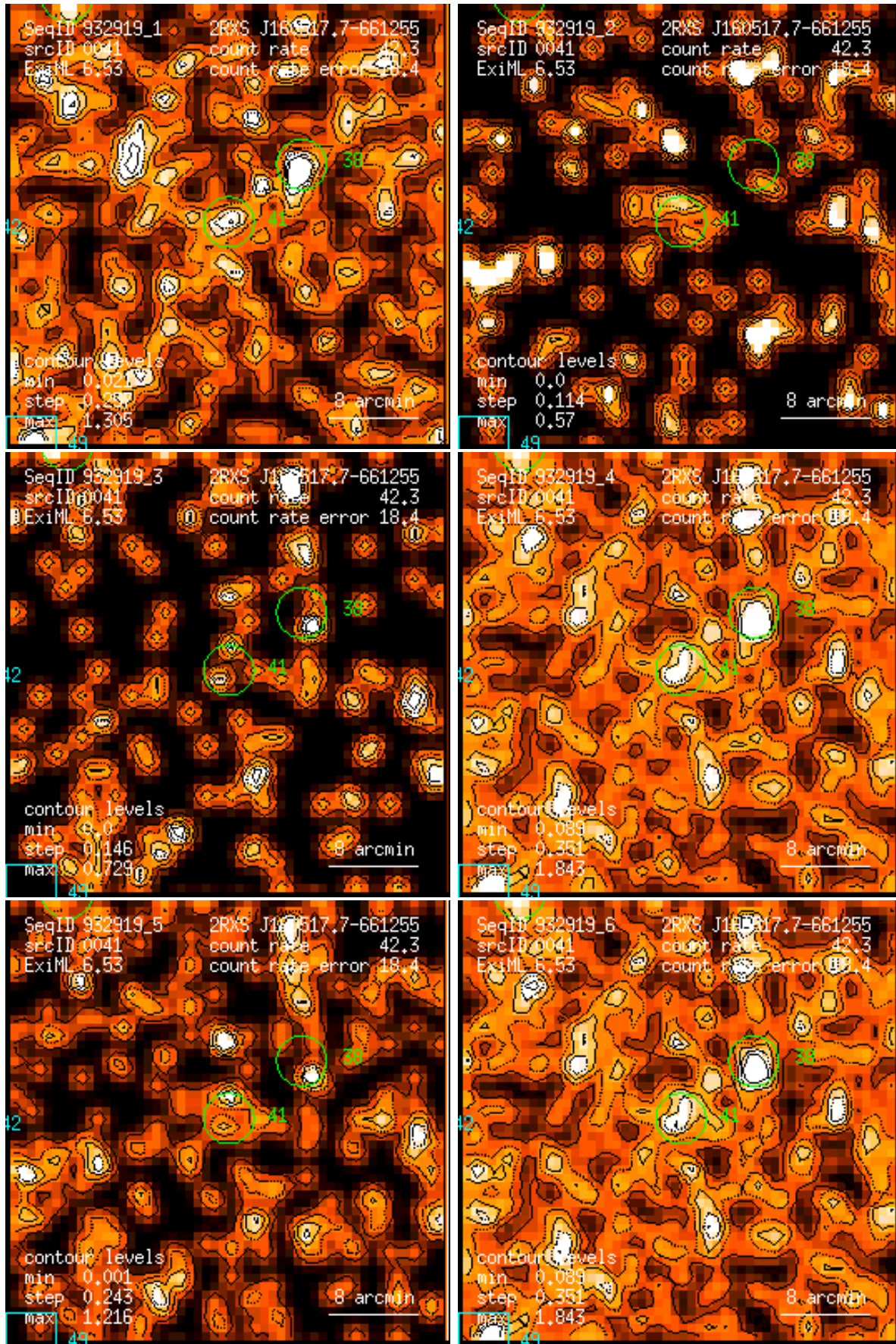
Figure 41: RASS 932919: detection 0041: band rate images, Gaussian filter: (1) PSPC channels 11 – 41, (2) 52 – 90, (3) 91 – 201, (4) 11 – 235, (5) 52 – 201, (6) 11 – 201. Broad band rates in counts/ks. Band rate contour levels in counts/ks/arcmin 2 .
