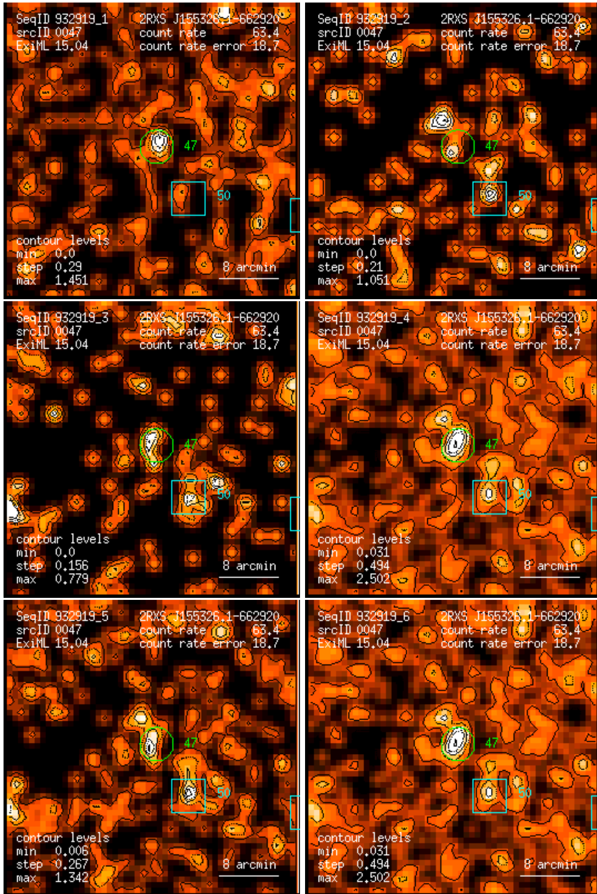
Figure 47: RASS 932919: detection 0047: band rate images, Gaussian filter: (1) PSPC channels 11 – 41, (2) 52 – 90, (3) 91 – 201, (4) 11 – 235, (5) 52 – 201, (6) 11 – 201. Broad band rates in counts/ks. Band rate contour levels in counts/ks/arcmin 2 .
