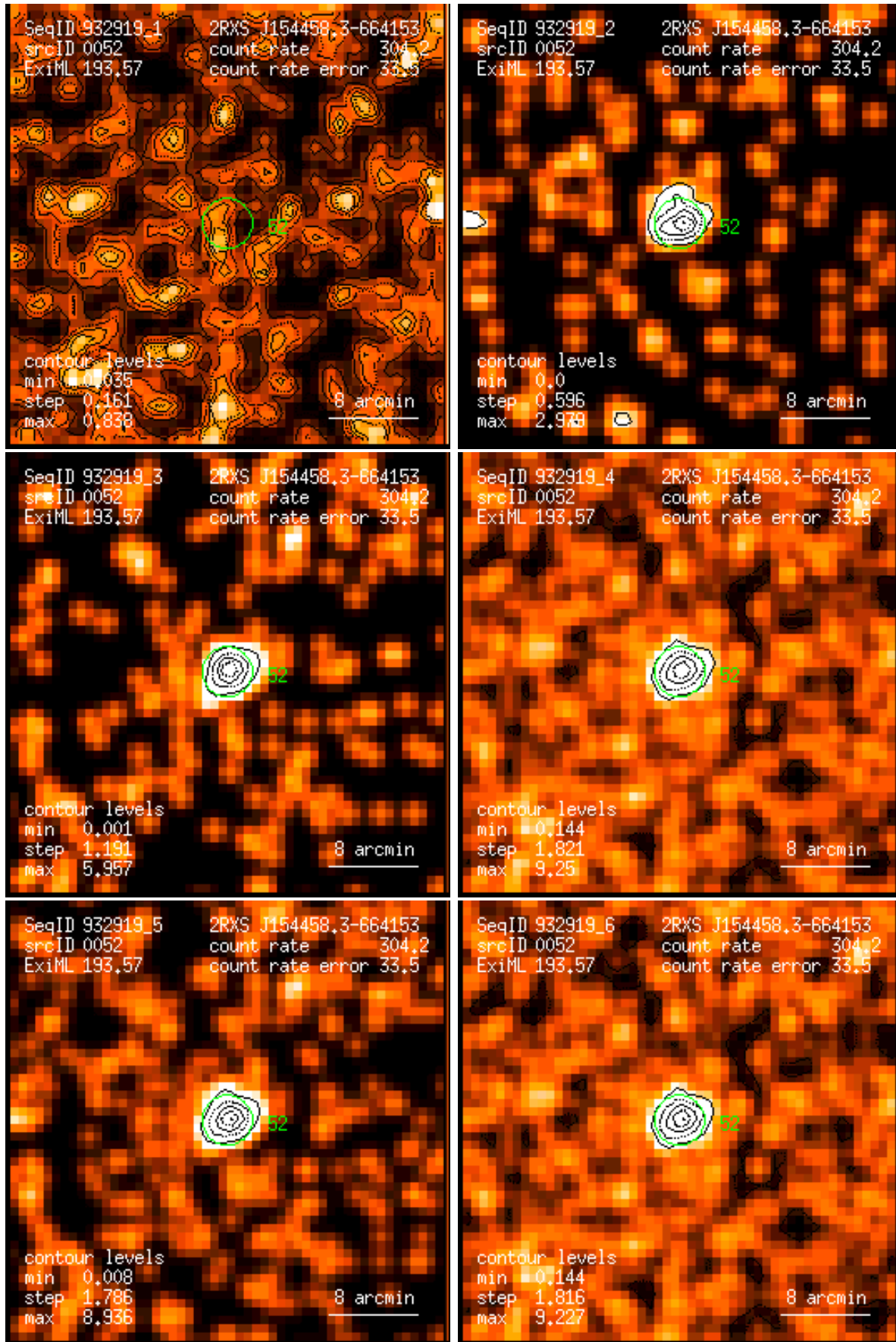
Figure 52: RASS 932919: detection 0052: band rate images, Gaussian filter: (1) PSPC channels 11 – 41, (2) 52 – 90, (3) 91 – 201, (4) 11 – 235, (5) 52 – 201, (6) 11 – 201. Broad band rates in counts/ks. Band rate contour levels in counts/ks/arcmin 2 .
