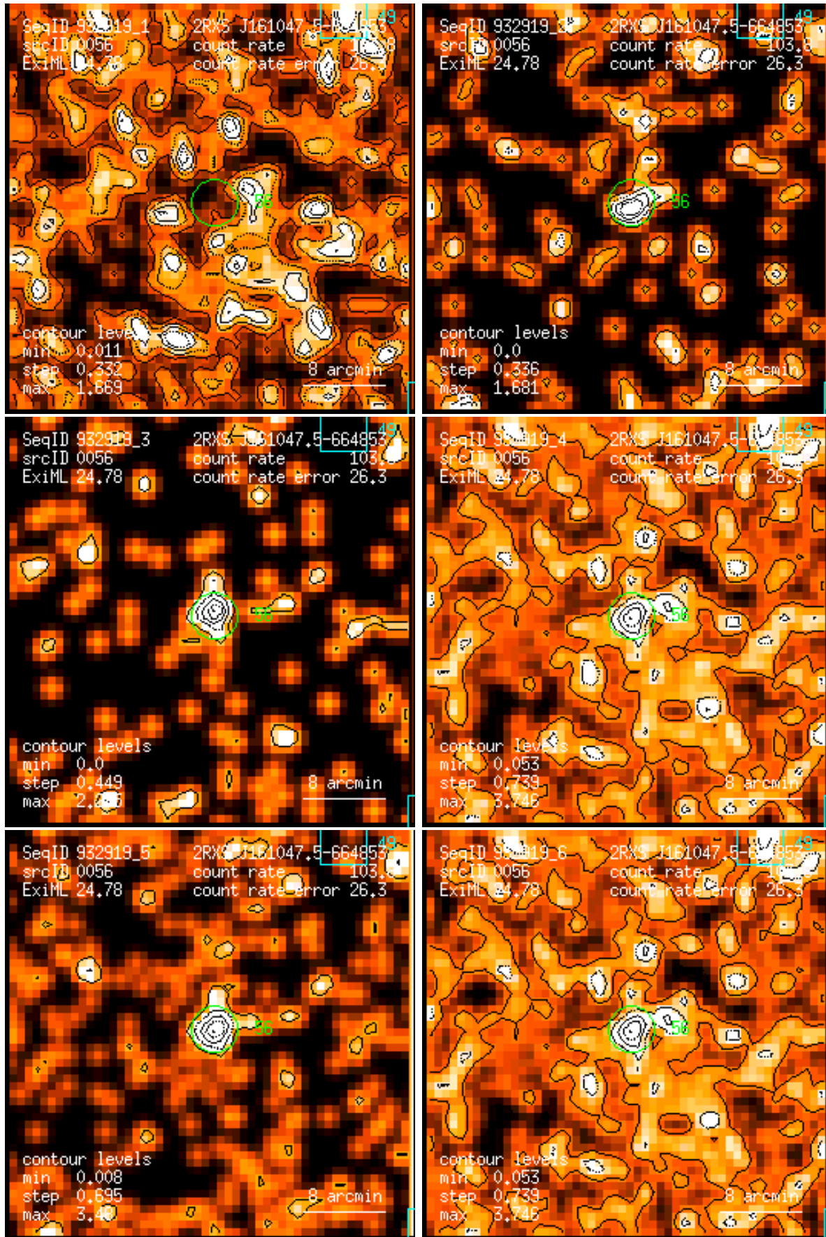
Figure 56: RASS 932919: detection 0056: band rate images, Gaussian filter: (1) PSPC channels 11 – 41, (2) 52 – 90, (3) 91 – 201, (4) 11 – 235, (5) 52 – 201, (6) 11 – 201. Broad band rates in counts/ks. Band rate contour levels in counts/ks/arcmin 2 .
