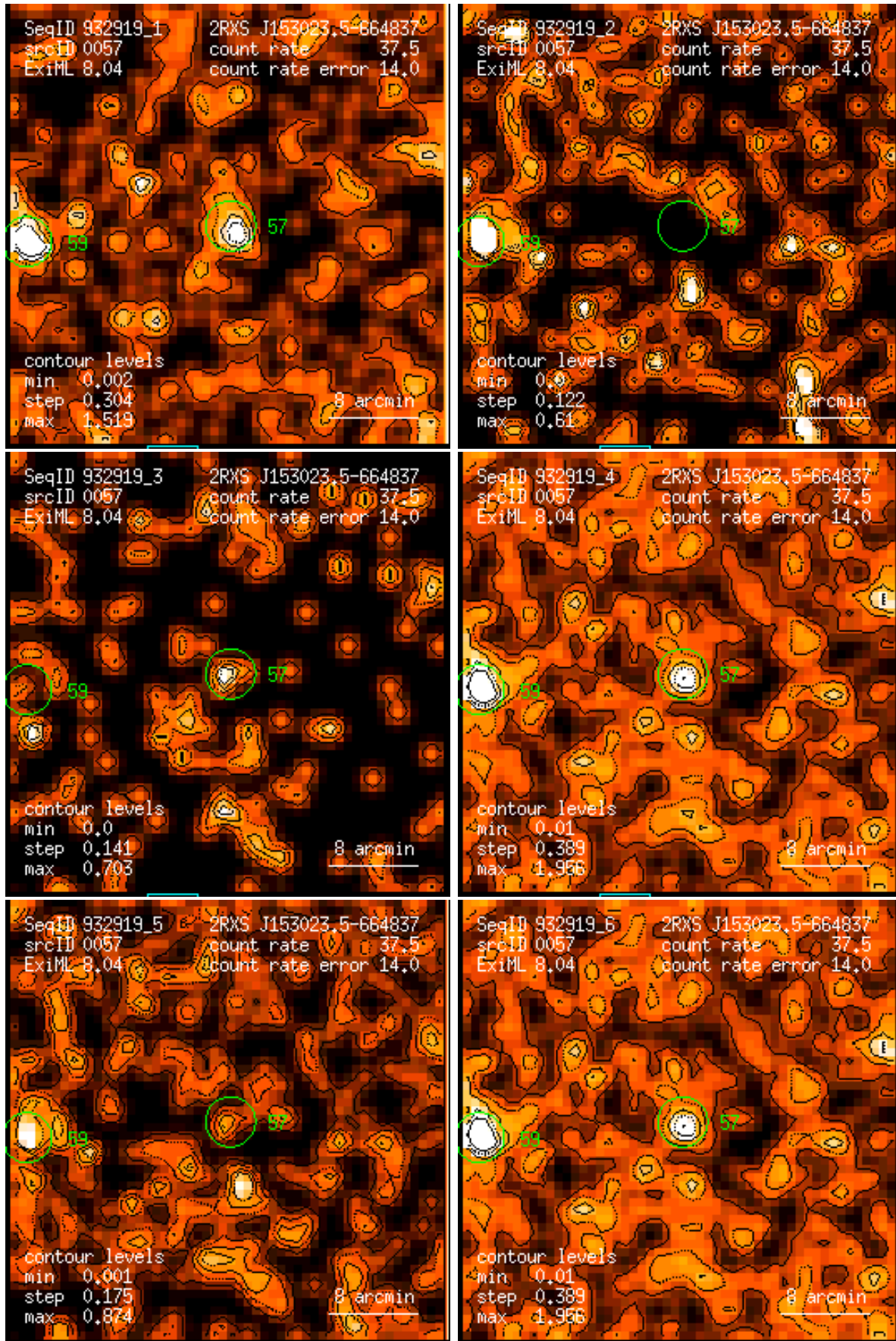
Figure 57: RASS 932919: detection 0057: band rate images, Gaussian filter: (1) PSPC channels 11 – 41, (2) 52 – 90, (3) 91 – 201, (4) 11 – 235, (5) 52 – 201, (6) 11 – 201. Broad band rates in counts/ks. Band rate contour levels in counts/ks/arcmin 2 .
