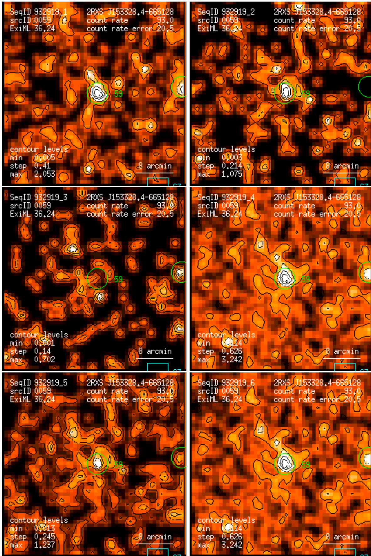
Figure 59: RASS 932919: detection 0059: band rate images, Gaussian filter: (1) PSPC channels 11 – 41, (2) 52 – 90, (3) 91 – 201, (4) 11 – 235, (5) 52 – 201, (6) 11 – 201. Broad band rates in counts/ks. Band rate contour levels in counts/ks/arcmin 2 .
