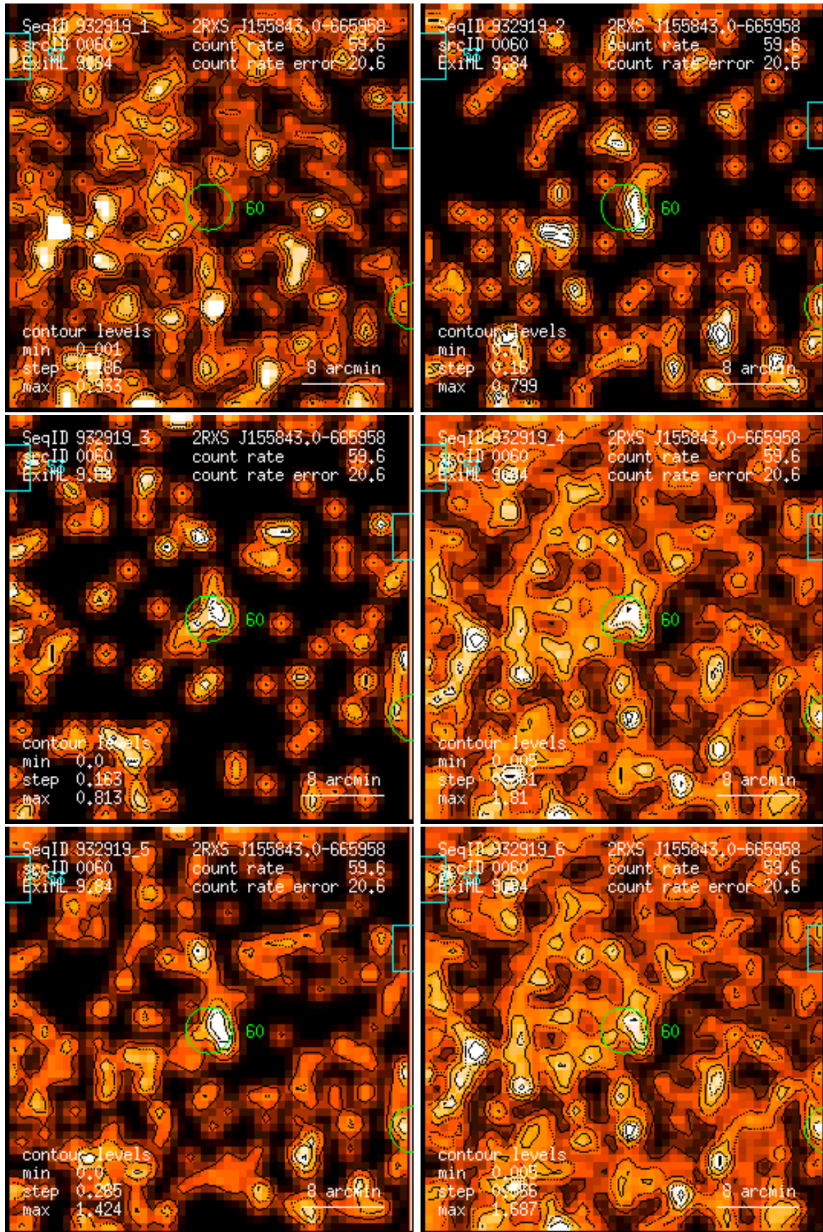
Figure 60: RASS 932919: detection 0060: band rate images, Gaussian filter: (1) PSPC channels 11 – 41, (2) 52 – 90, (3) 91 – 201, (4) 11 – 235, (5) 52 – 201, (6) 11 – 201. Broad band rates in counts/ks. Band rate contour levels in counts/ks/arcmin 2 .
