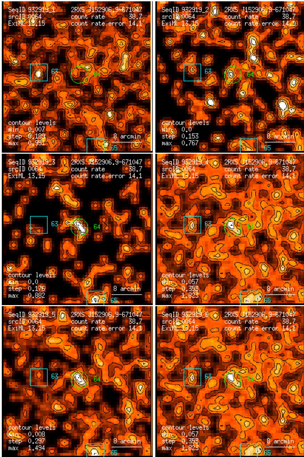
Figure 64: RASS 932919: detection 0064: band rate images, Gaussian filter: (1) PSPC channels 11 – 41, (2) 52 – 90, (3) 91 – 201, (4) 11 – 235, (5) 52 – 201, (6) 11 – 201. Broad band rates in counts/ks. Band rate contour levels in counts/ks/arcmin 2 .
