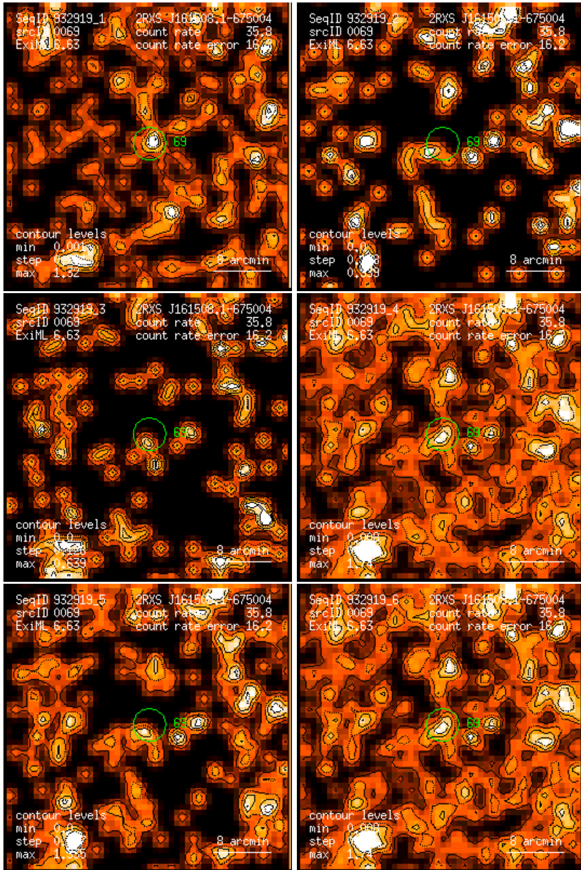
Figure 69: RASS 932919: detection 0069: band rate images, Gaussian filter: (1) PSPC channels 11 – 41, (2) 52 – 90, (3) 91 – 201, (4) 11 – 235, (5) 52 – 201, (6) 11 – 201. Broad band rates in counts/ks. Band rate contour levels in counts/ks/arcmin 2 .
