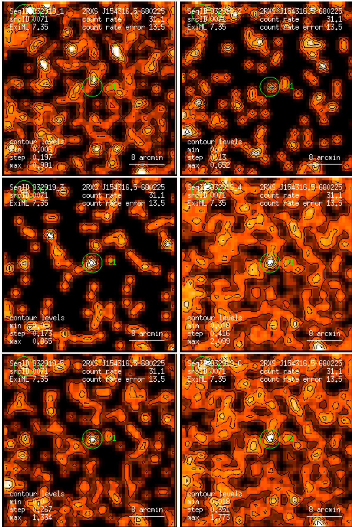
Figure 71: RASS 932919: detection 0071: band rate images, Gaussian filter: (1) PSPC channels 11 – 41, (2) 52 – 90, (3) 91 – 201, (4) 11 – 235, (5) 52 – 201, (6) 11 – 201. Broad band rates in counts/ks. Band rate contour levels in counts/ks/arcmin 2 .
