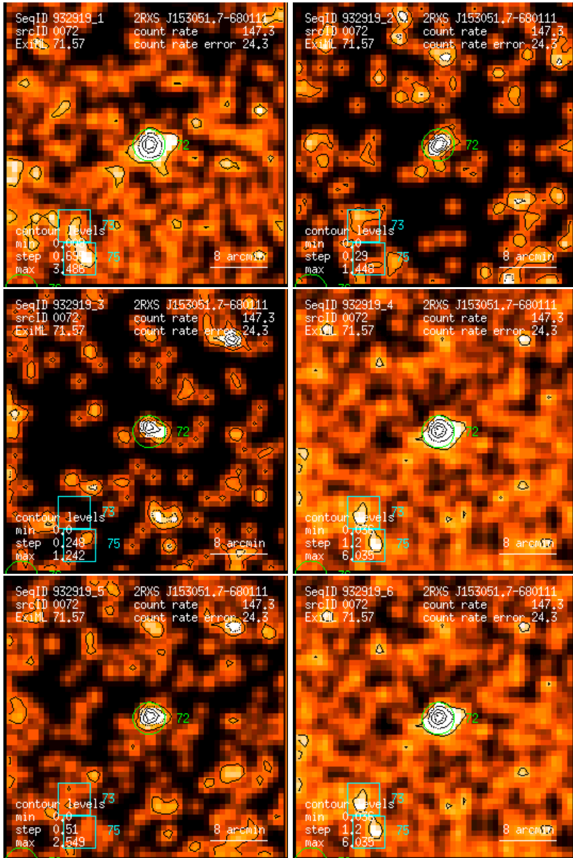
Figure 72: RASS 932919: detection 0072: band rate images, Gaussian filter: (1) PSPC channels 11 – 41, (2) 52 – 90, (3) 91 – 201, (4) 11 – 235, (5) 52 – 201, (6) 11 – 201. Broad band rates in counts/ks. Band rate contour levels in counts/ks/arcmin 2 .
