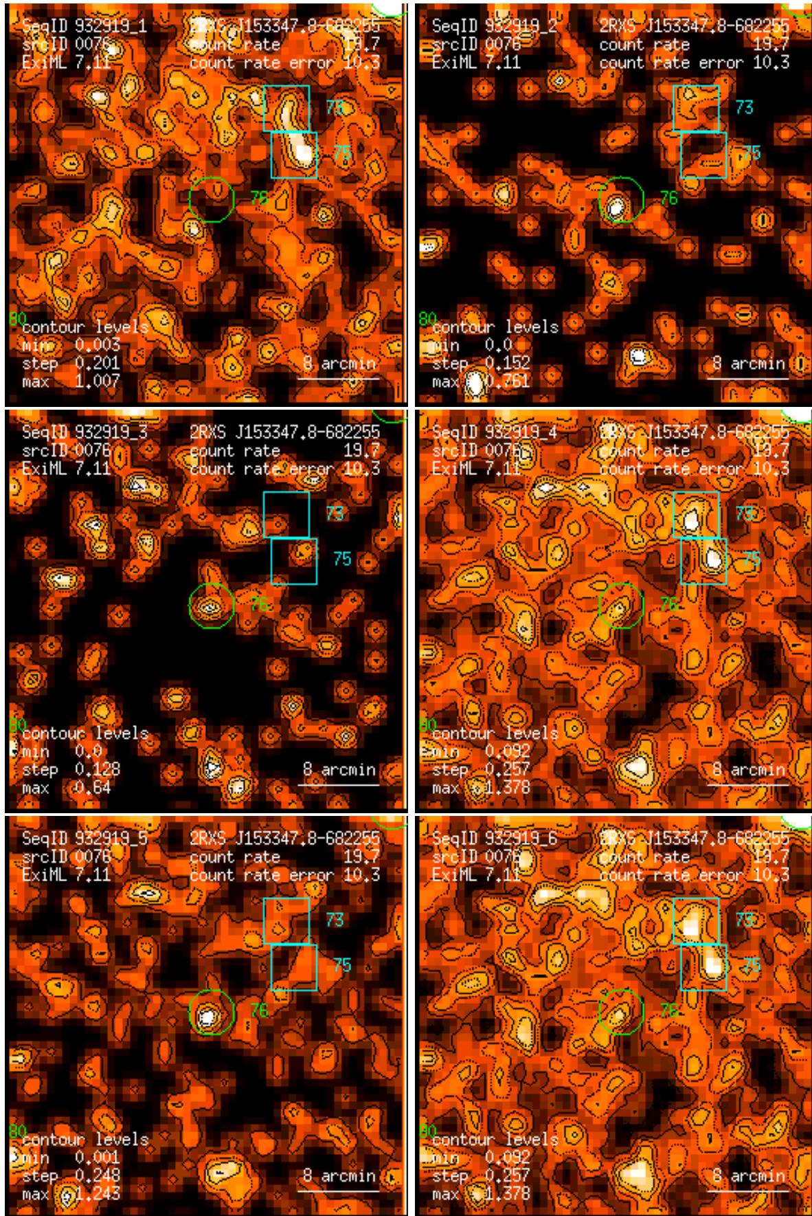
Figure 76: RASS 932919: detection 0076: band rate images, Gaussian filter: (1) PSPC channels 11 – 41, (2) 52 – 90, (3) 91 – 201, (4) 11 – 235, (5) 52 – 201, (6) 11 – 201. Broad band rates in counts/ks. Band rate contour levels in counts/ks/arcmin 2 .
