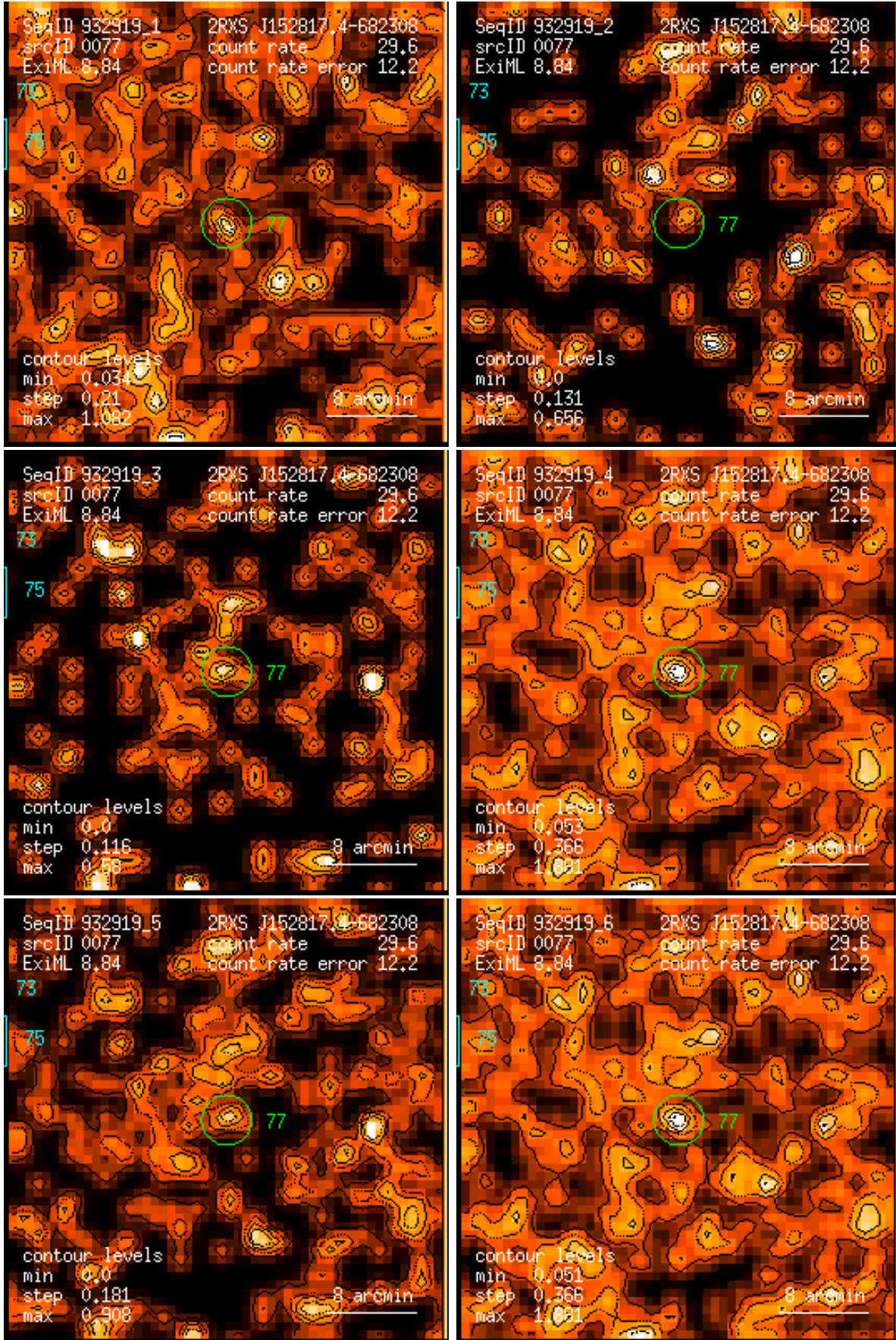
Figure 77: RASS 932919: detection 0077: band rate images, Gaussian filter: (1) PSPC channels 11 – 41, (2) 52 – 90, (3) 91 – 201, (4) 11 – 235, (5) 52 – 201, (6) 11 – 201. Broad band rates in counts/ks. Band rate contour levels in counts/ks/arcmin 2 .
