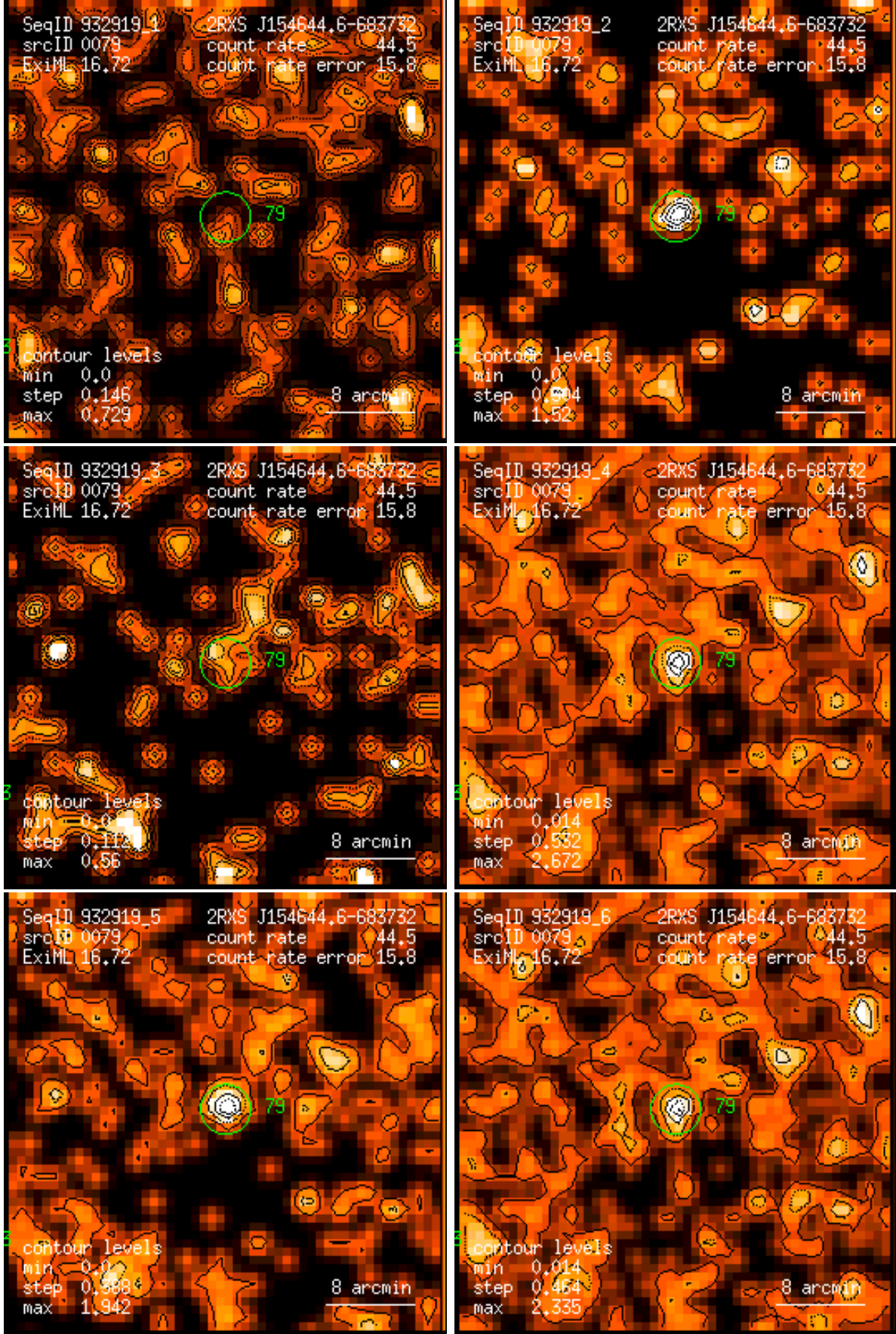
Figure 79: RASS 932919: detection 0079: band rate images, Gaussian filter: (1) PSPC channels 11 – 41, (2) 52 – 90, (3) 91 – 201, (4) 11 – 235, (5) 52 – 201, (6) 11 – 201. Broad band rates in counts/ks. Band rate contour levels in counts/ks/arcmin 2 .
