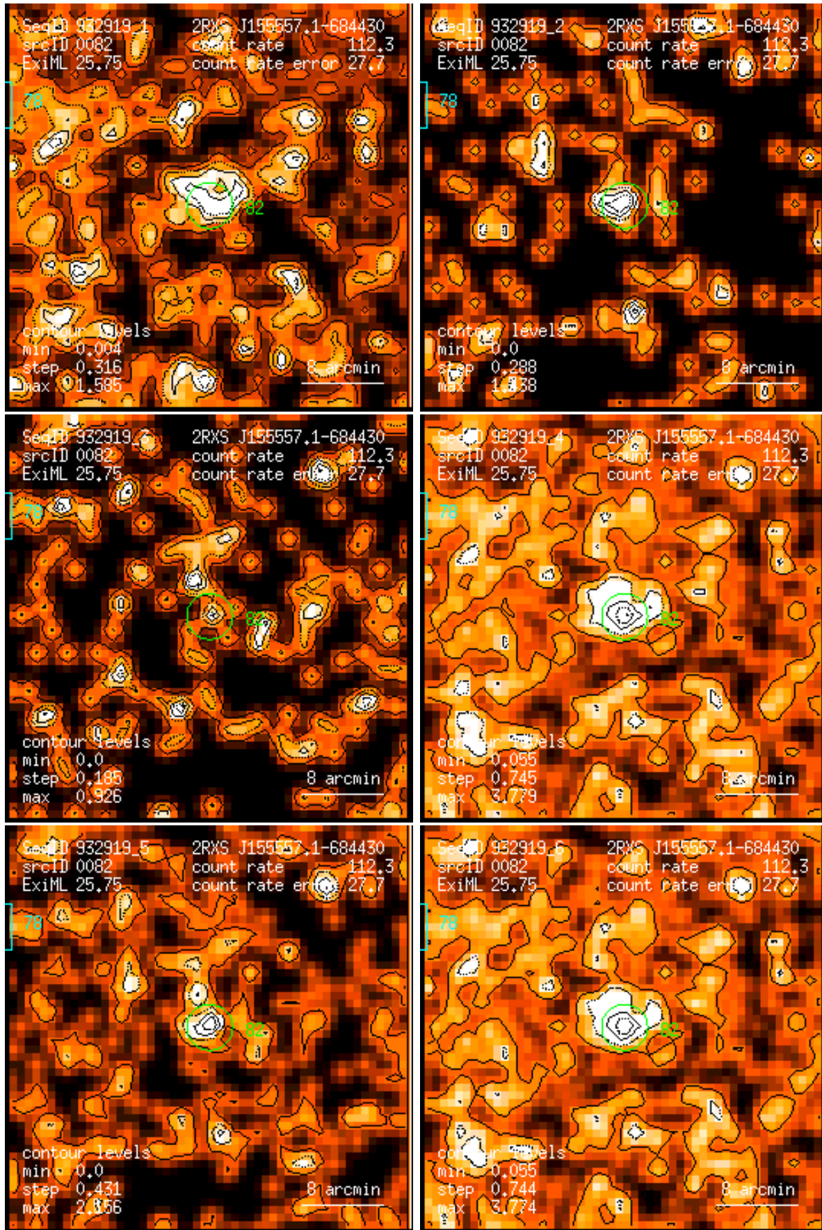
Figure 82: RASS 932919: detection 0082: band rate images, Gaussian filter: (1) PSPC channels 11 – 41, (2) 52 – 90, (3) 91 – 201, (4) 11 – 235, (5) 52 – 201, (6) 11 – 201. Broad band rates in counts/ks. Band rate contour levels in counts/ks/arcmin 2 .
