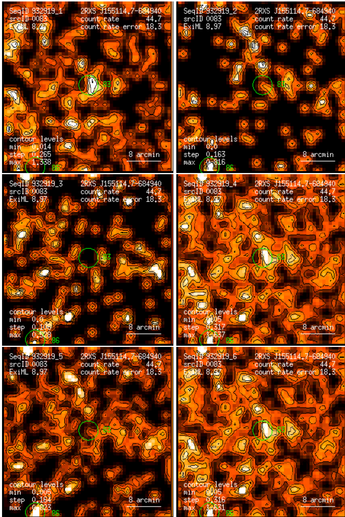
Figure 83: RASS 932919: detection 0083: band rate images, Gaussian filter: (1) PSPC channels 11 – 41, (2) 52 – 90, (3) 91 – 201, (4) 11 – 235, (5) 52 – 201, (6) 11 – 201. Broad band rates in counts/ks. Band rate contour levels in counts/ks/arcmin 2 .
