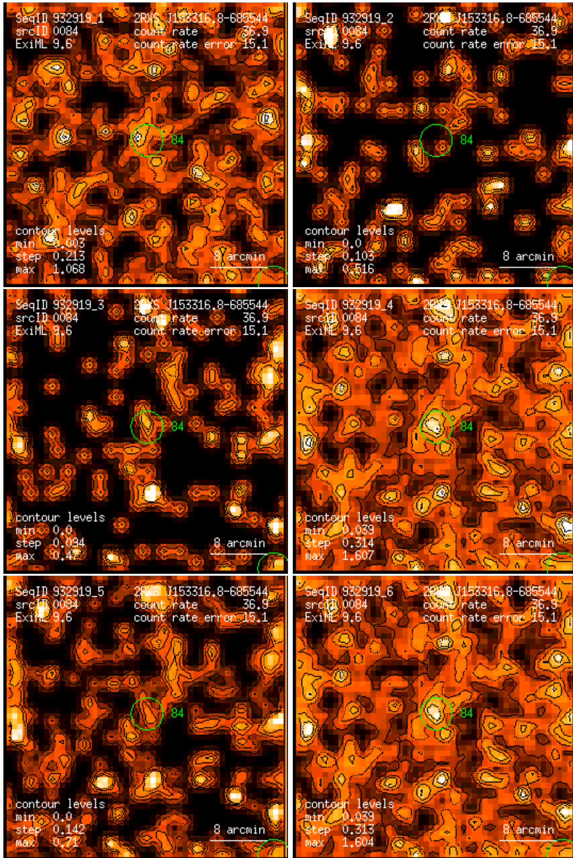
Figure 84: RASS 932919: detection 0084: band rate images, Gaussian filter: (1) PSPC channels 11 – 41, (2) 52 – 90, (3) 91 – 201, (4) 11 – 235, (5) 52 – 201, (6) 11 – 201. Broad band rates in counts/ks. Band rate contour levels in counts/ks/arcmin 2 .
