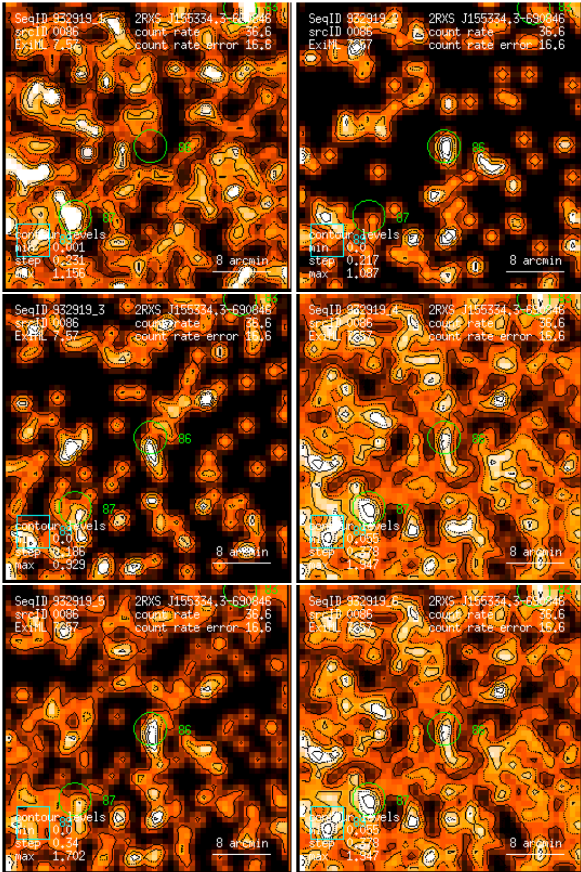
Figure 86: RASS 932919: detection 0086: band rate images, Gaussian filter: (1) PSPC channels 11 – 41, (2) 52 – 90, (3) 91 – 201, (4) 11 – 235, (5) 52 – 201, (6) 11 – 201. Broad band rates in counts/ks. Band rate contour levels in counts/ks/arcmin 2 .
