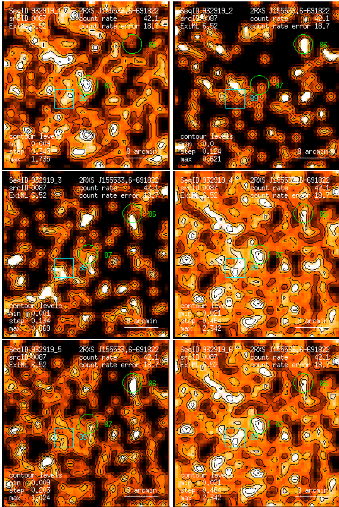
Figure 87: RASS 932919: detection 0087: band rate images, Gaussian filter: (1) PSPC channels 11 – 41, (2) 52 – 90, (3) 91 – 201, (4) 11 – 235, (5) 52 – 201, (6) 11 – 201. Broad band rates in counts/ks. Band rate contour levels in counts/ks/arcmin 2 .
