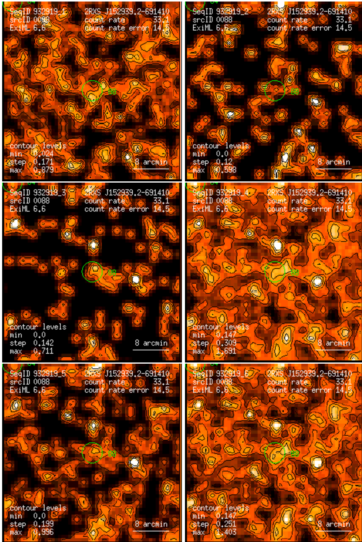
Figure 88: RASS 932919: detection 0088: band rate images, Gaussian filter: (1) PSPC channels 11 – 41, (2) 52 – 90, (3) 91 – 201, (4) 11 – 235, (5) 52 – 201, (6) 11 – 201. Broad band rates in counts/ks. Band rate contour levels in counts/ks/arcmin 2 .
