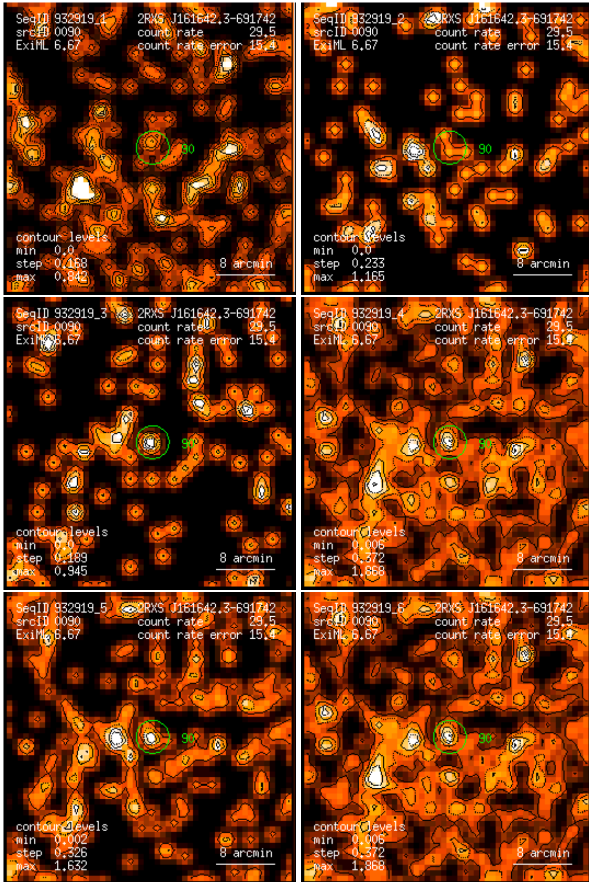
Figure 90: RASS 932919: detection 0090: band rate images, Gaussian filter: (1) PSPC channels 11 – 41, (2) 52 – 90, (3) 91 – 201, (4) 11 – 235, (5) 52 – 201, (6) 11 – 201. Broad band rates in counts/ks. Band rate contour levels in counts/ks/arcmin 2 .
