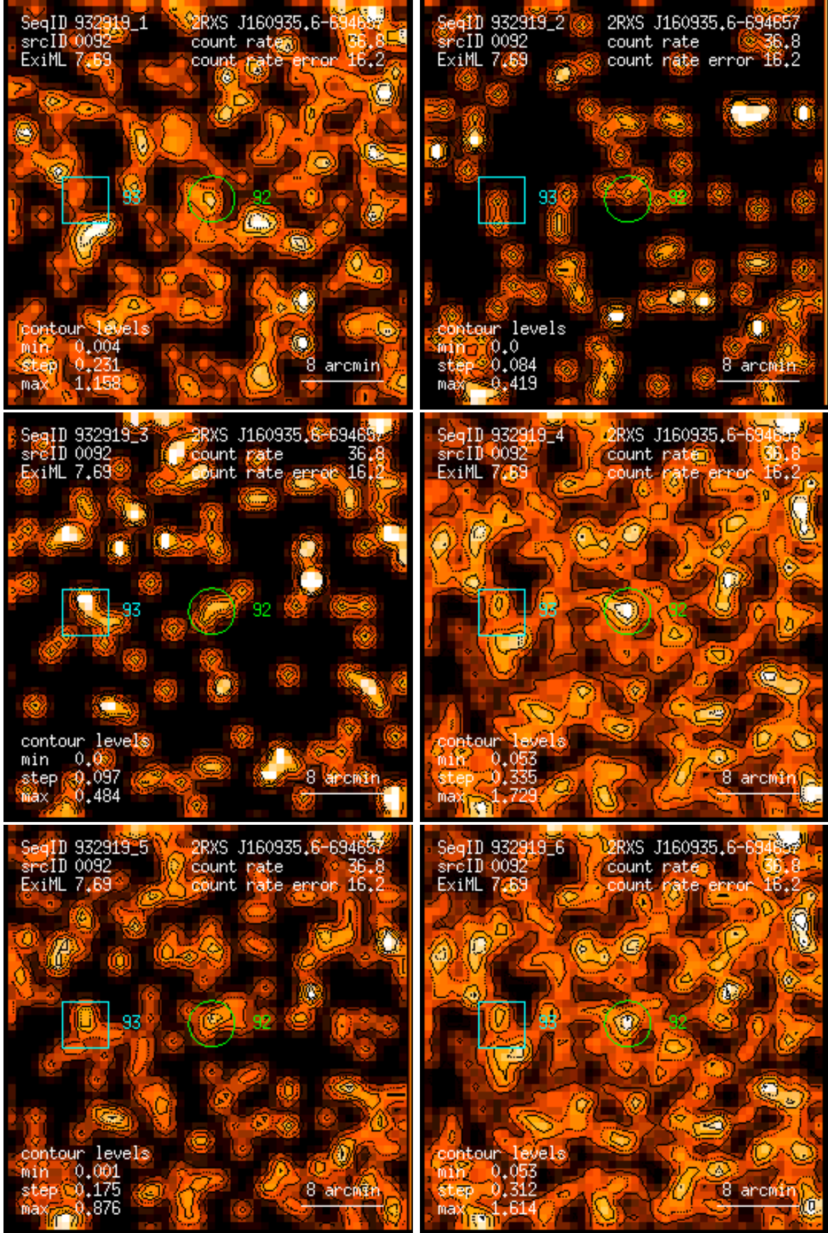
Figure 92: RASS 932919: detection 0092: band rate images, Gaussian filter: (1) PSPC channels 11 – 41, (2) 52 – 90, (3) 91 – 201, (4) 11 – 235, (5) 52 – 201, (6) 11 – 201. Broad band rates in counts/ks. Band rate contour levels in counts/ks/arcmin 2 .
