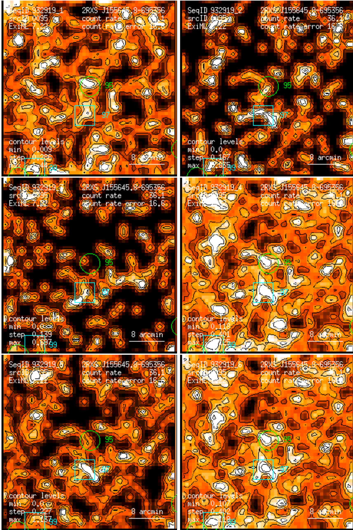
Figure 95: RASS 932919: detection 0095: band rate images, Gaussian filter: (1) PSPC channels 11 – 41, (2) 52 – 90, (3) 91 – 201, (4) 11 – 235, (5) 52 – 201, (6) 11 – 201. Broad band rates in counts/ks. Band rate contour levels in counts/ks/arcmin 2 .
