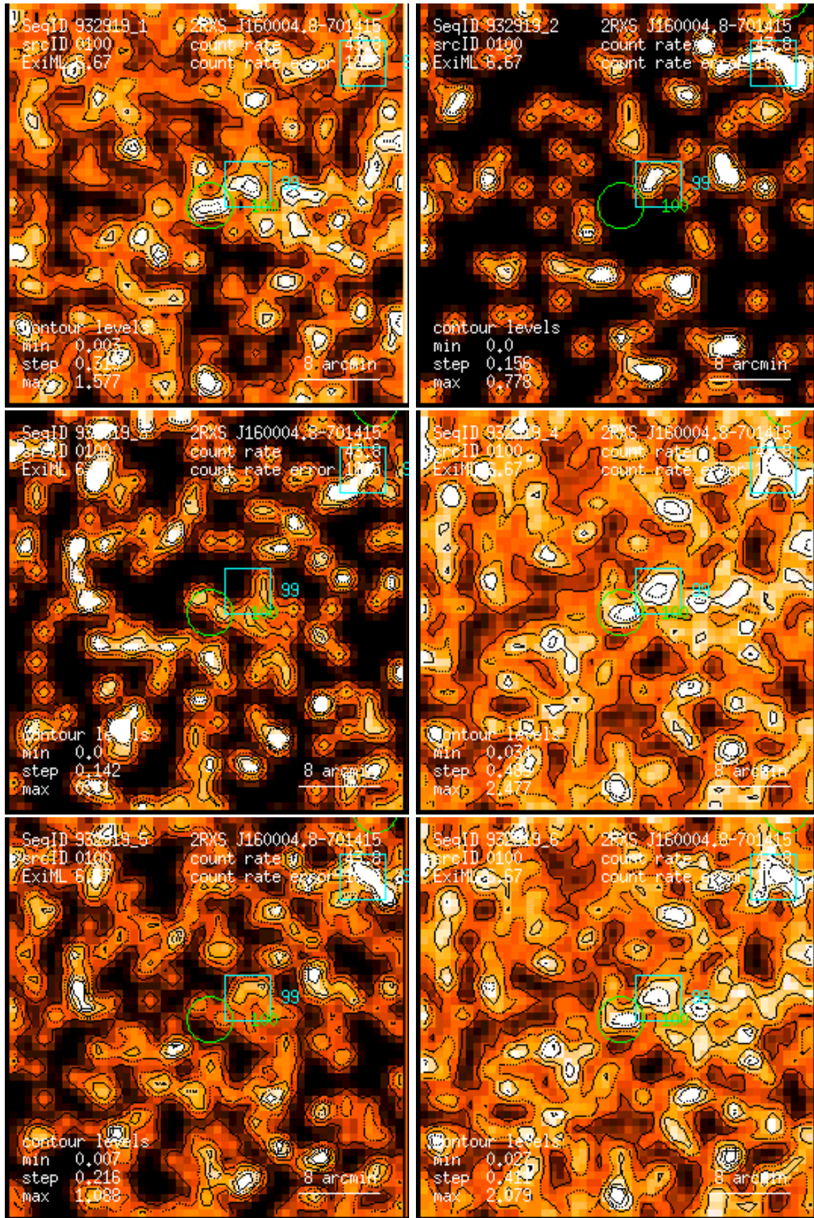
Figure 100: RASS 932919: detection 0100: band rate images, Gaussian filter: (1) PSPC channels 11 – 41, (2) 52 – 90, (3) 91 – 201, (4) 11 – 235, (5) 52 – 201, (6) 11 – 201. Broad band rates in counts/ks. Band rate contour levels in counts/ks/arcmin 2 .
