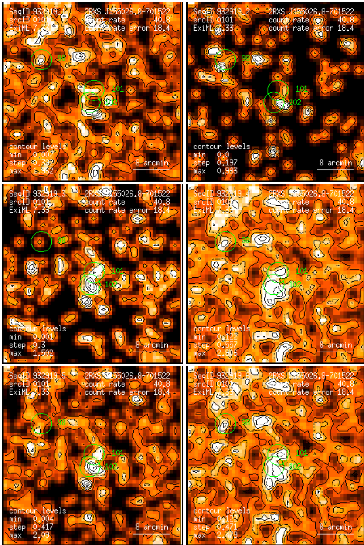
Figure 101: RASS 932919: detection 0101: band rate images, Gaussian filter: (1) PSPC channels 11 – 41, (2) 52 – 90, (3) 91 – 201, (4) 11 – 235, (5) 52 – 201, (6) 11 – 201. Broad band rates in counts/ks. Band rate contour levels in counts/ks/arcmin 2 .
