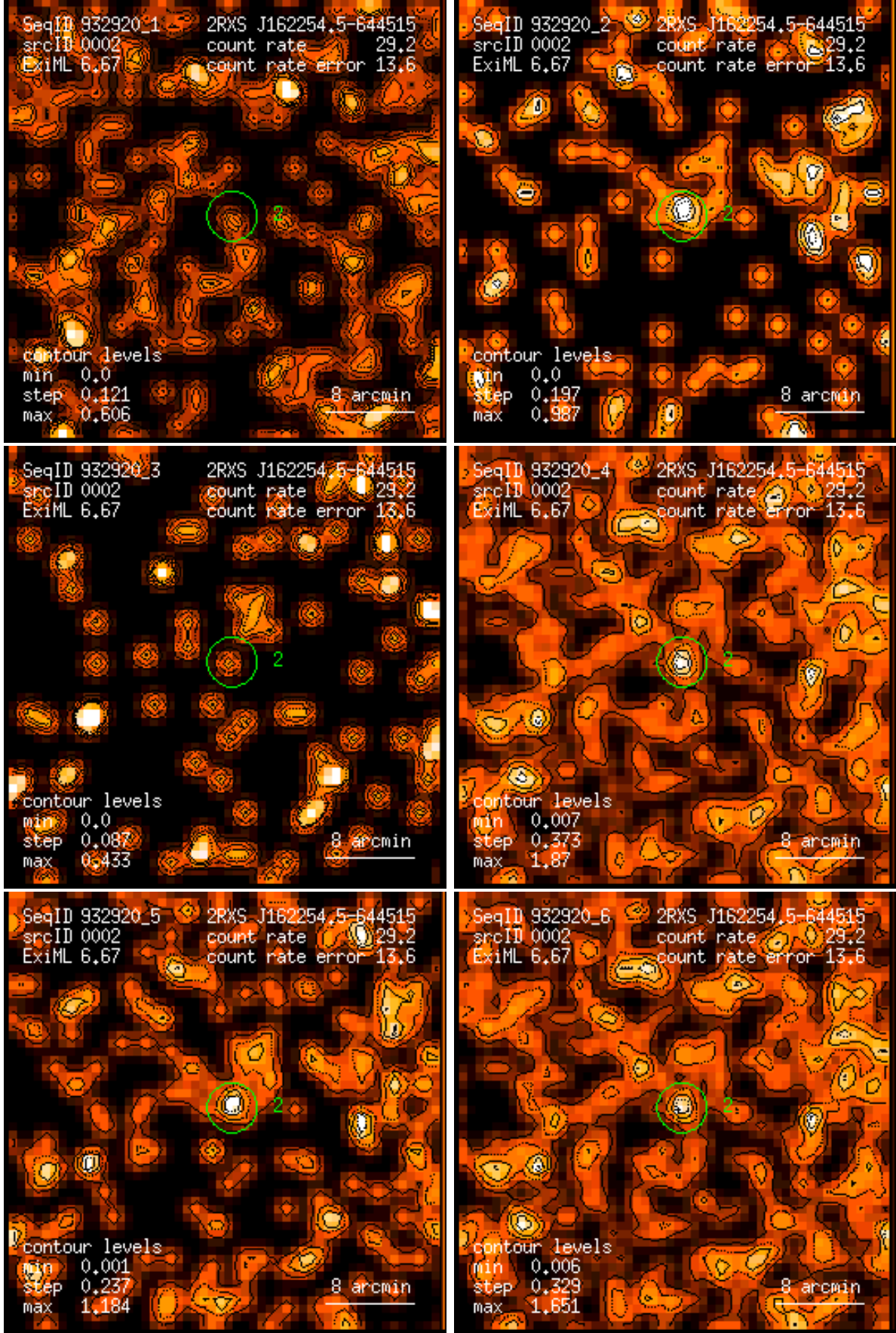
Figure 2: RASS 932920: detection 0002: band rate images, Gaussian filter: (1) PSPC channels 11 – 41, (2) 52 – 90, (3) 91 – 201, (4) 11 – 235, (5) 52 – 201, (6) 11 – 201. Broad band rates in counts/ks. Band rate contour levels in counts/ks/arcmin 2 .
