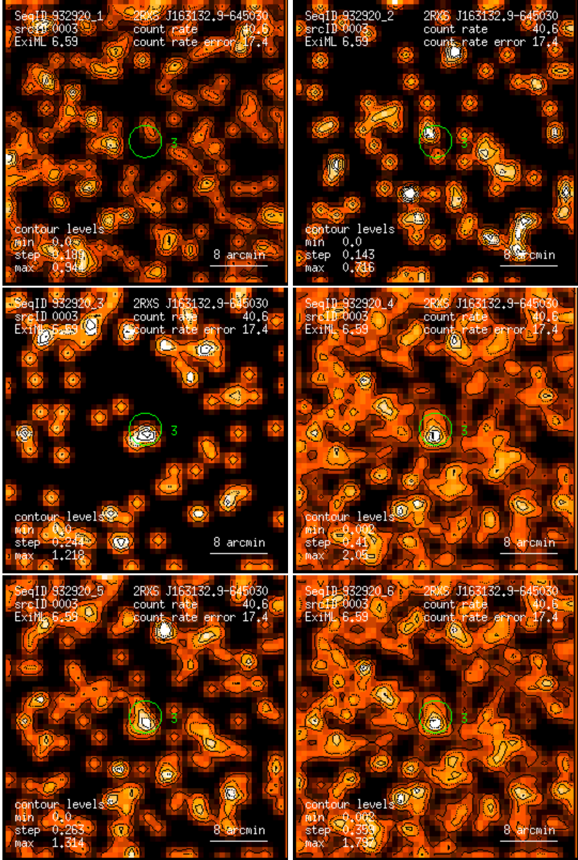
Figure 3: RASS 932920: detection 0003: band rate images, Gaussian filter: (1) PSPC channels 11 – 41, (2) 52 – 90, (3) 91 – 201, (4) 11 – 235, (5) 52 – 201, (6) 11 – 201. Broad band rates in counts/ks. Band rate contour levels in counts/ks/arcmin 2 .
