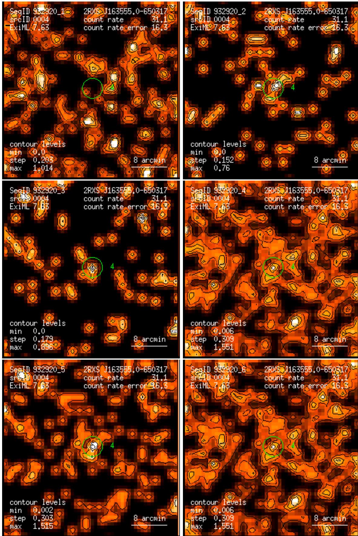
Figure 4: RASS 932920: detection 0004: band rate images, Gaussian filter: (1) PSPC channels 11 – 41, (2) 52 – 90, (3) 91 – 201, (4) 11 – 235, (5) 52 – 201, (6) 11 – 201. Broad band rates in counts/ks. Band rate contour levels in counts/ks/arcmin 2 .
