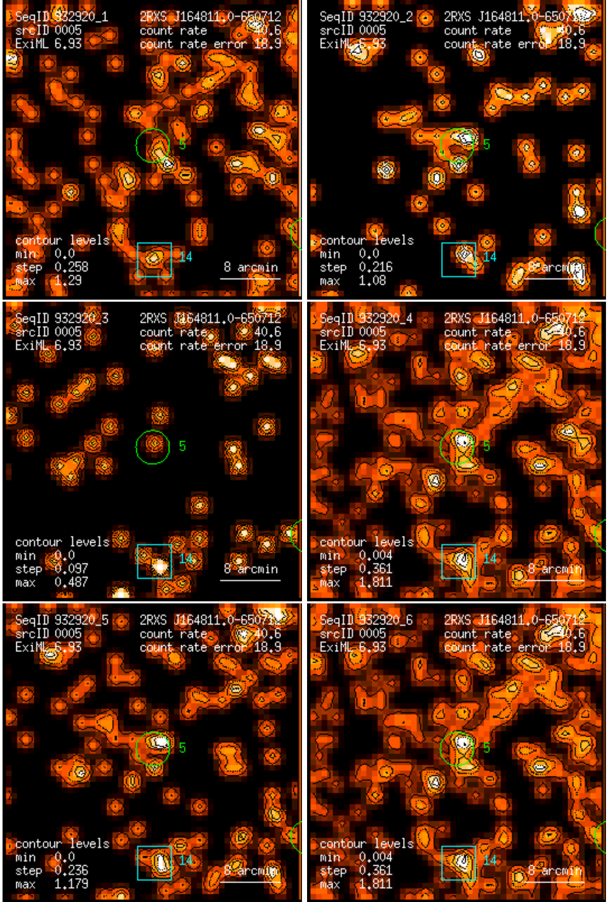
Figure 5: RASS 932920: detection 0005: band rate images, Gaussian filter: (1) PSPC channels 11 – 41, (2) 52 – 90, (3) 91 – 201, (4) 11 – 235, (5) 52 – 201, (6) 11 – 201. Broad band rates in counts/ks. Band rate contour levels in counts/ks/arcmin 2 .
