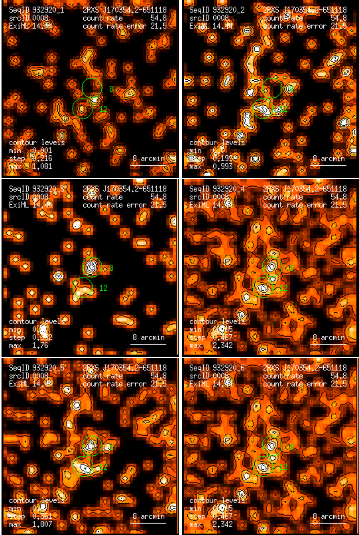
Figure 8: RASS 932920: detection 0008: band rate images, Gaussian filter: (1) PSPC channels 11 – 41, (2) 52 – 90, (3) 91 – 201, (4) 11 – 235, (5) 52 – 201, (6) 11 – 201. Broad band rates in counts/ks. Band rate contour levels in counts/ks/arcmin 2 .
