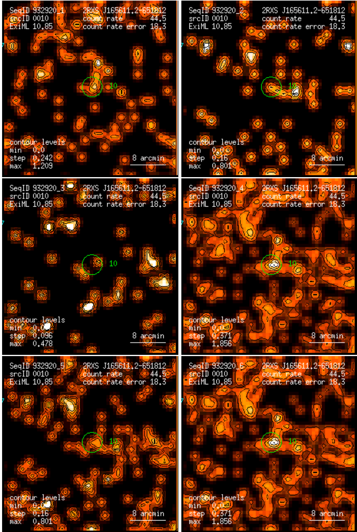
Figure 10: RASS 932920: detection 0010: band rate images, Gaussian filter: (1) PSPC channels 11 – 41, (2) 52 – 90, (3) 91 – 201, (4) 11 – 235, (5) 52 – 201, (6) 11 – 201. Broad band rates in counts/ks. Band rate contour levels in counts/ks/arcmin 2 .
