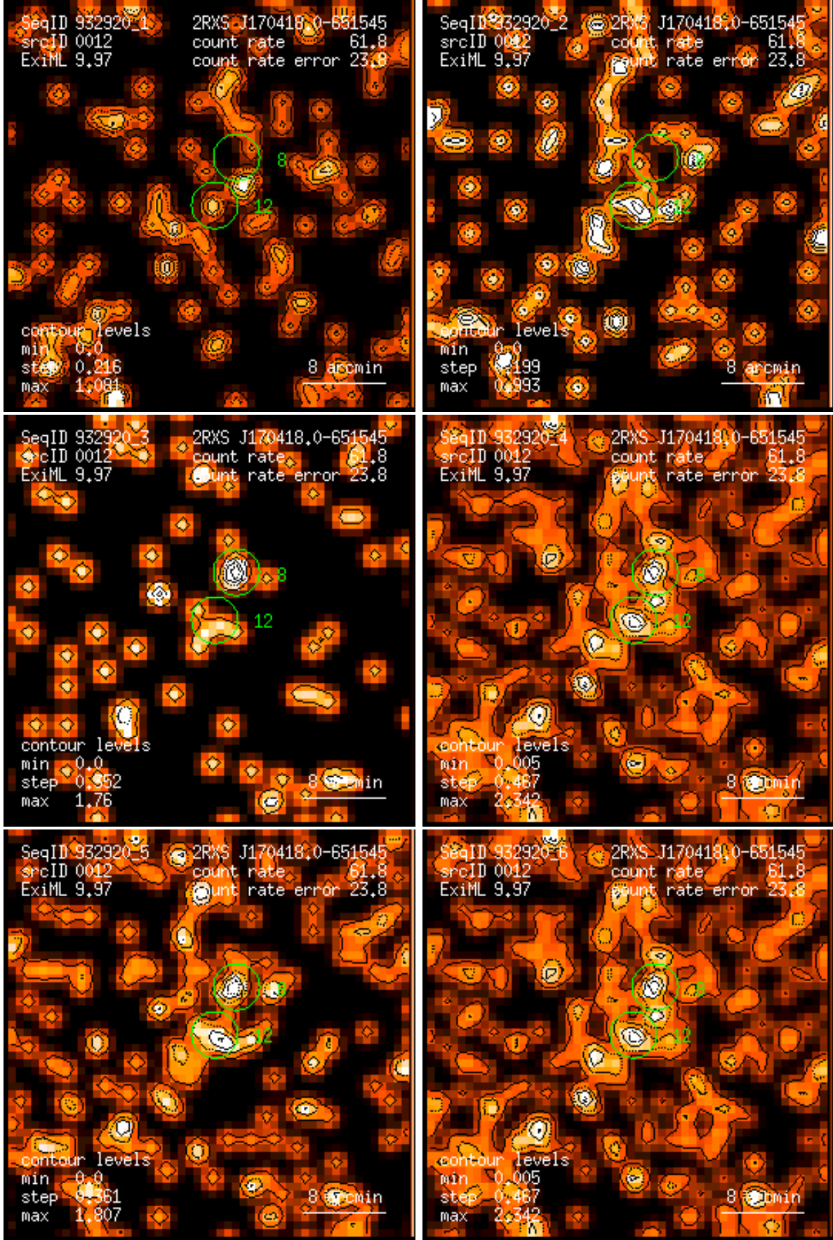
Figure 12: RASS 932920: detection 0012: band rate images, Gaussian filter: (1) PSPC channels 11 – 41, (2) 52 – 90, (3) 91 – 201, (4) 11 – 235, (5) 52 – 201, (6) 11 – 201. Broad band rates in counts/ks. Band rate contour levels in counts/ks/arcmin 2 .
