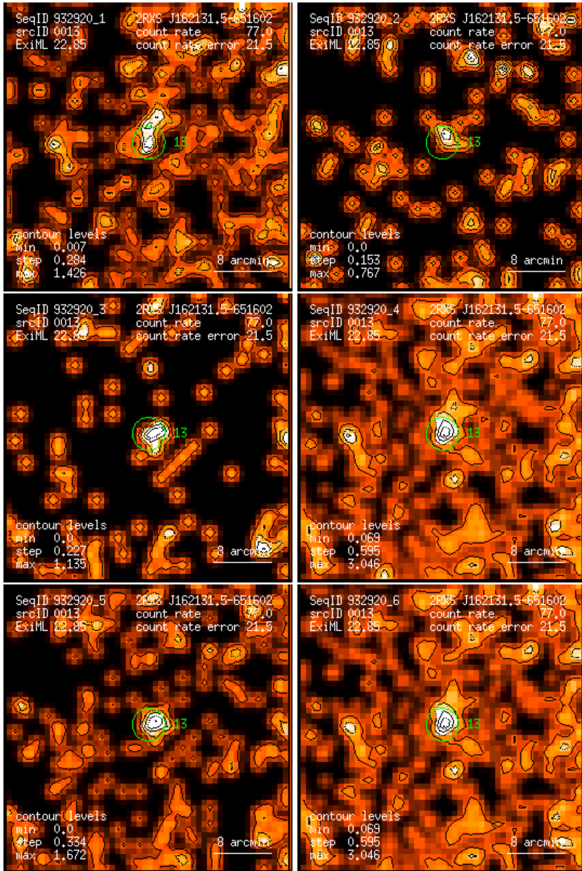
Figure 13: RASS 932920: detection 0013: band rate images, Gaussian filter: (1) PSPC channels 11 – 41, (2) 52 – 90, (3) 91 – 201, (4) 11 – 235, (5) 52 – 201, (6) 11 – 201. Broad band rates in counts/ks. Band rate contour levels in counts/ks/arcmin 2 .
