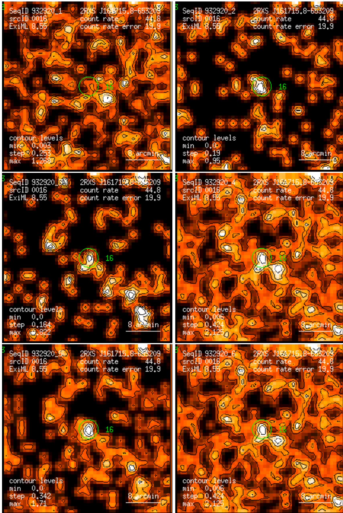
Figure 16: RASS 932920: detection 0016: band rate images, Gaussian filter: (1) PSPC channels 11 – 41, (2) 52 – 90, (3) 91 – 201, (4) 11 – 235, (5) 52 – 201, (6) 11 – 201. Broad band rates in counts/ks. Band rate contour levels in counts/ks/arcmin 2 .
