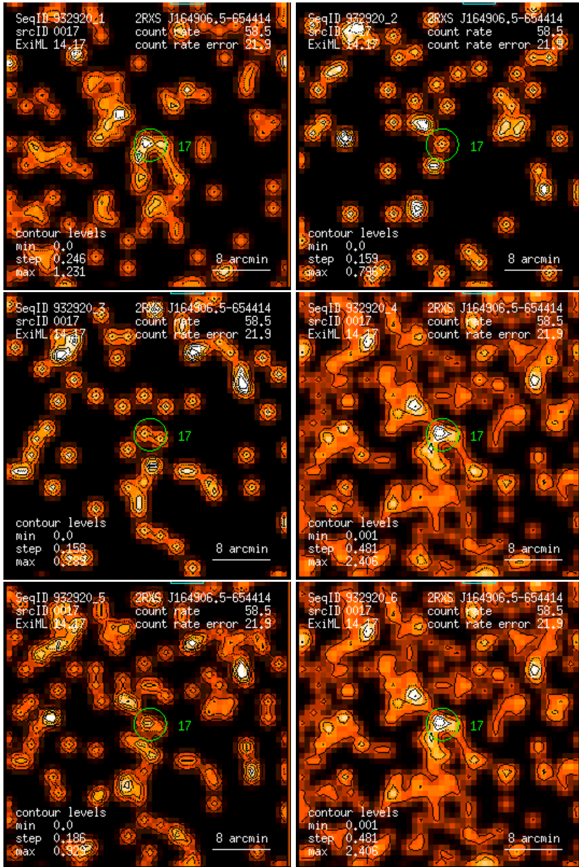
Figure 17: RASS 932920: detection 0017: band rate images, Gaussian filter: (1) PSPC channels 11 – 41, (2) 52 – 90, (3) 91 – 201, (4) 11 – 235, (5) 52 – 201, (6) 11 – 201. Broad band rates in counts/ks. Band rate contour levels in counts/ks/arcmin 2 .
