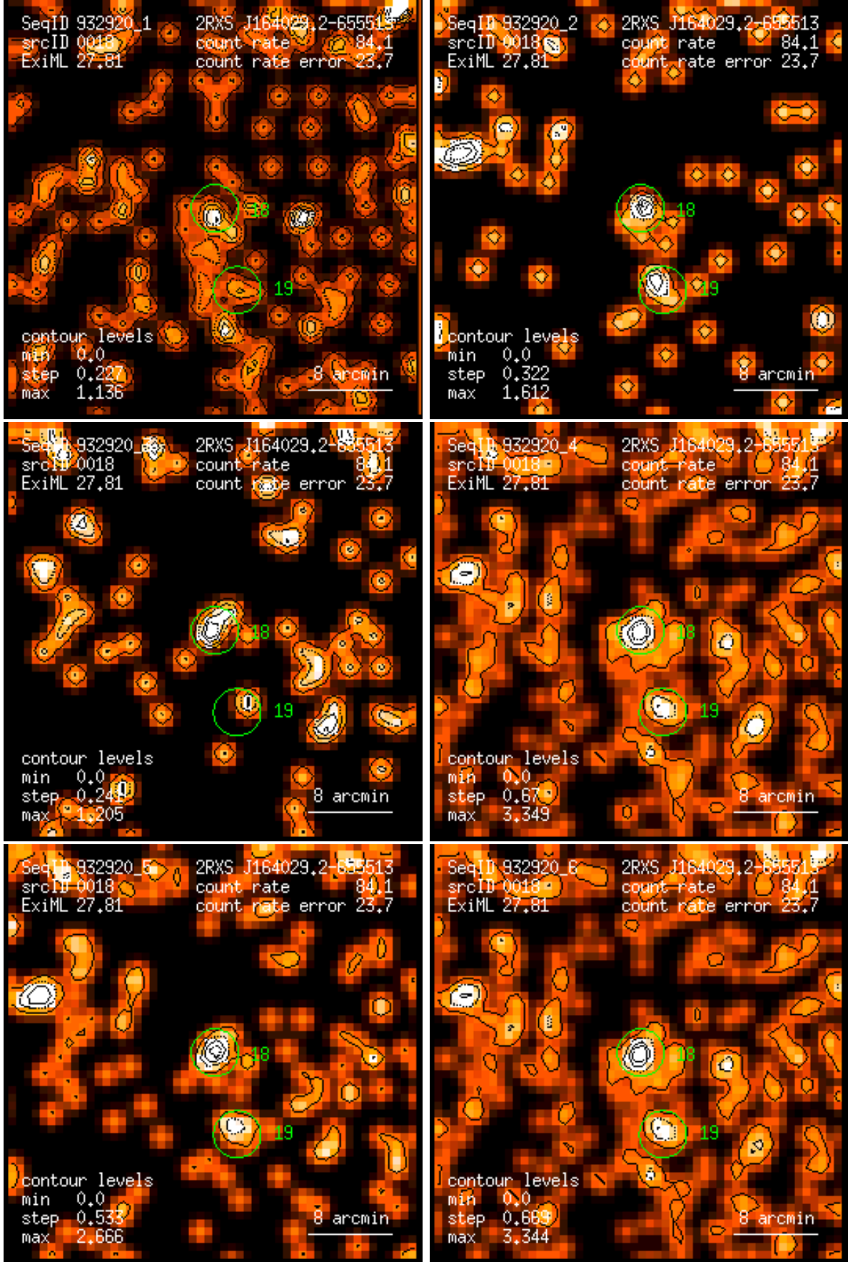
Figure 18: RASS 932920: detection 0018: band rate images, Gaussian filter: (1) PSPC channels 11 – 41, (2) 52 – 90, (3) 91 – 201, (4) 11 – 235, (5) 52 – 201, (6) 11 – 201. Broad band rates in counts/ks. Band rate contour levels in counts/ks/arcmin 2 .
