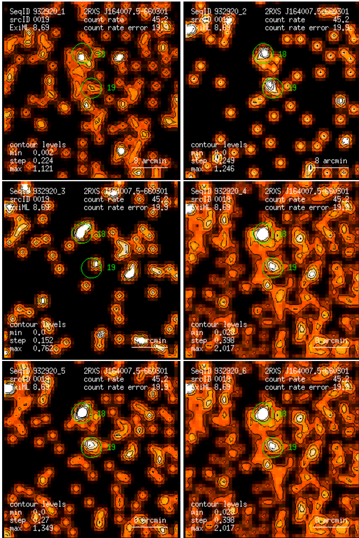
Figure 19: RASS 932920: detection 0019: band rate images, Gaussian filter: (1) PSPC channels 11 – 41, (2) 52 – 90, (3) 91 – 201, (4) 11 – 235, (5) 52 – 201, (6) 11 – 201. Broad band rates in counts/ks. Band rate contour levels in counts/ks/arcmin 2 .
