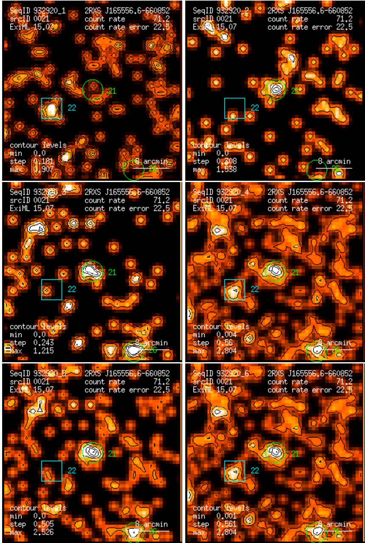
Figure 21: RASS 932920: detection 0021: band rate images, Gaussian filter: (1) PSPC channels 11 – 41, (2) 52 – 90, (3) 91 – 201, (4) 11 – 235, (5) 52 – 201, (6) 11 – 201. Broad band rates in counts/ks. Band rate contour levels in counts/ks/arcmin 2 .
