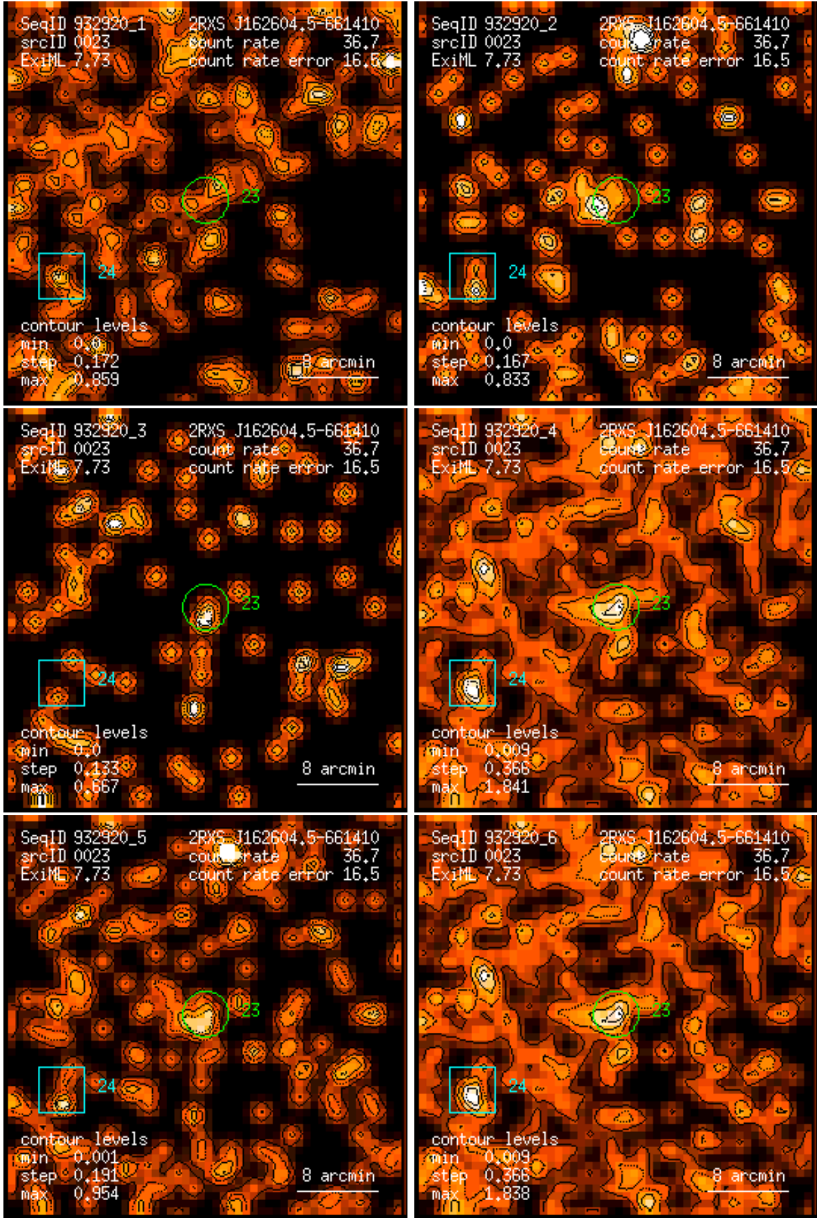
Figure 23: RASS 932920: detection 0023: band rate images, Gaussian filter: (1) PSPC channels 11 – 41, (2) 52 – 90, (3) 91 – 201, (4) 11 – 235, (5) 52 – 201, (6) 11 – 201. Broad band rates in counts/ks. Band rate contour levels in counts/ks/arcmin 2 .
