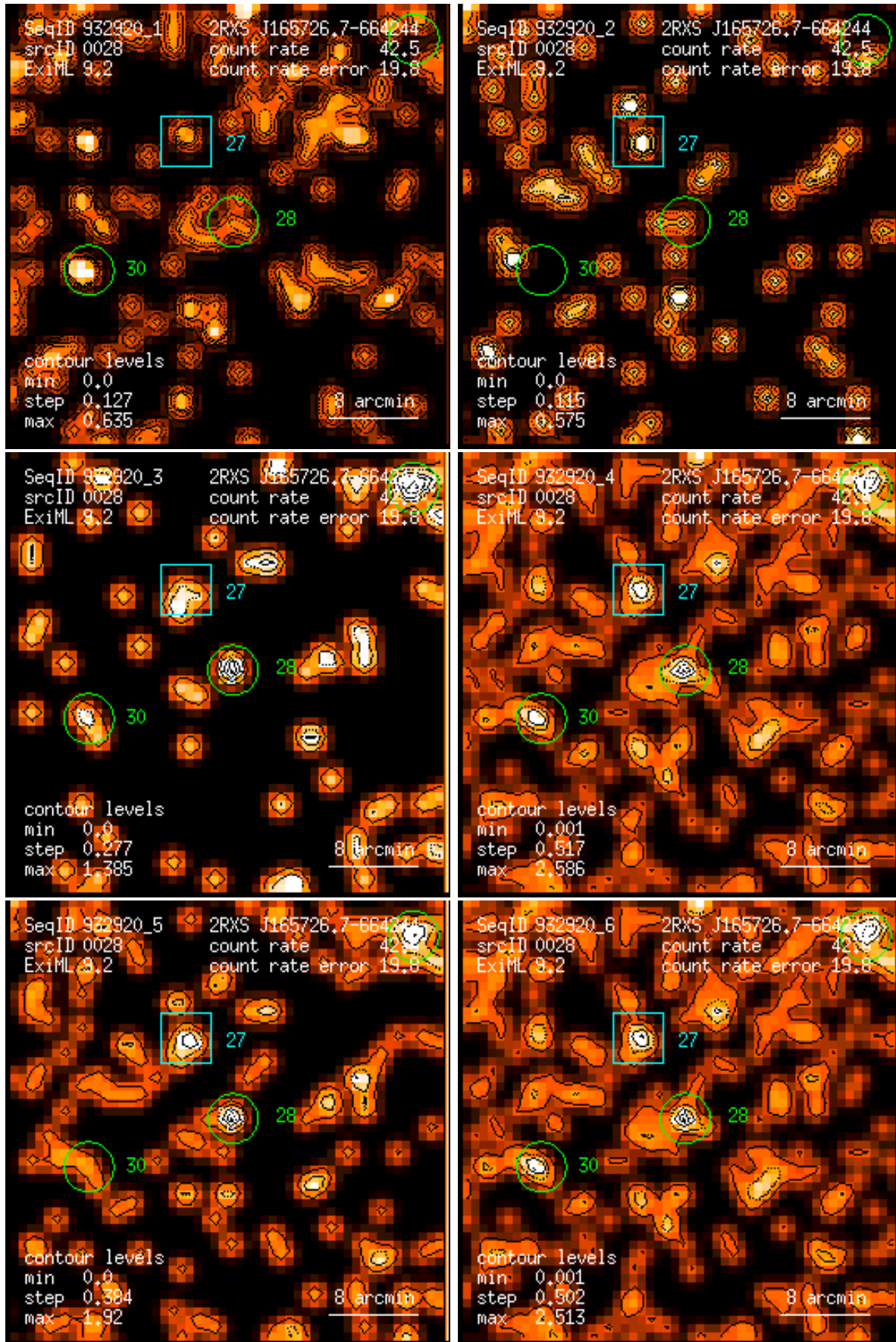
Figure 28: RASS 932920: detection 0028: band rate images, Gaussian filter: (1) PSPC channels 11 – 41, (2) 52 – 90, (3) 91 – 201, (4) 11 – 235, (5) 52 – 201, (6) 11 – 201. Broad band rates in counts/ks. Band rate contour levels in counts/ks/arcmin 2 .
