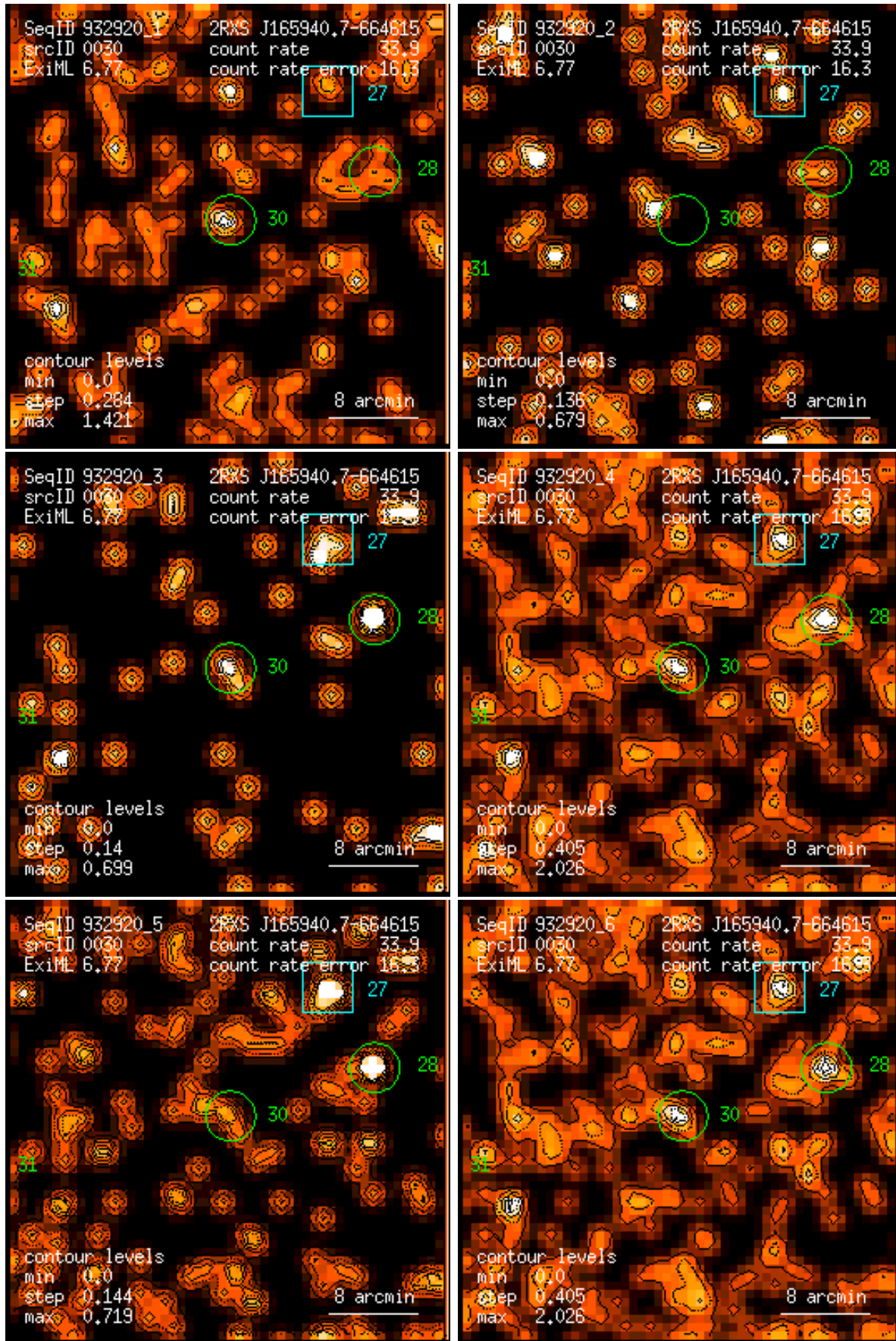
Figure 30: RASS 932920: detection 0030: band rate images, Gaussian filter: (1) PSPC channels 11 – 41, (2) 52 – 90, (3) 91 – 201, (4) 11 – 235, (5) 52 – 201, (6) 11 – 201. Broad band rates in counts/ks. Band rate contour levels in counts/ks/arcmin 2 .
