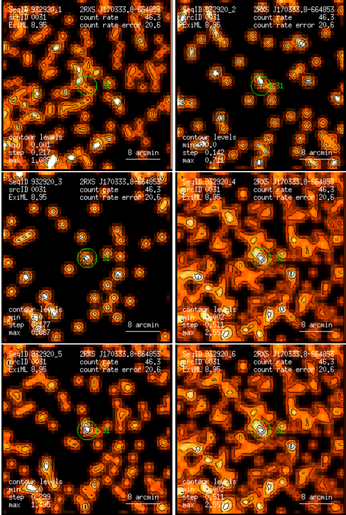
Figure 31: RASS 932920: detection 0031: band rate images, Gaussian filter: (1) PSPC channels 11 – 41, (2) 52 – 90, (3) 91 – 201, (4) 11 – 235, (5) 52 – 201, (6) 11 – 201. Broad band rates in counts/ks. Band rate contour levels in counts/ks/arcmin 2 .
