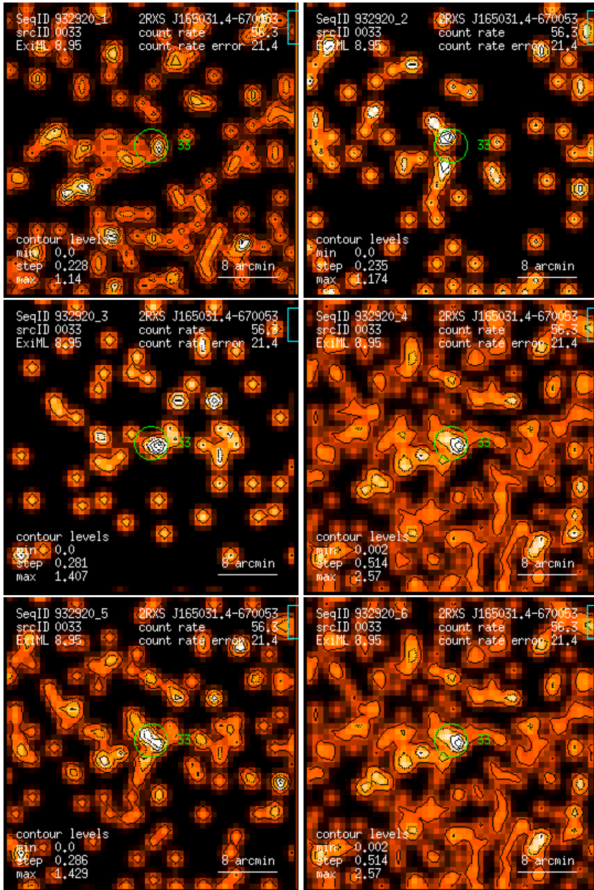
Figure 33: RASS 932920: detection 0033: band rate images, Gaussian filter: (1) PSPC channels 11 – 41, (2) 52 – 90, (3) 91 – 201, (4) 11 – 235, (5) 52 – 201, (6) 11 – 201. Broad band rates in counts/ks. Band rate contour levels in counts/ks/arcmin 2 .
