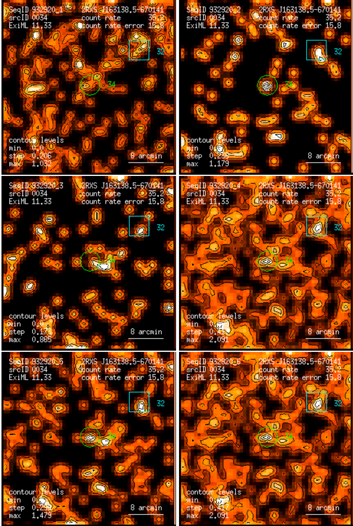
Figure 34: RASS 932920: detection 0034: band rate images, Gaussian filter: (1) PSPC channels 11 – 41, (2) 52 – 90, (3) 91 – 201, (4) 11 – 235, (5) 52 – 201, (6) 11 – 201. Broad band rates in counts/ks. Band rate contour levels in counts/ks/arcmin 2 .
