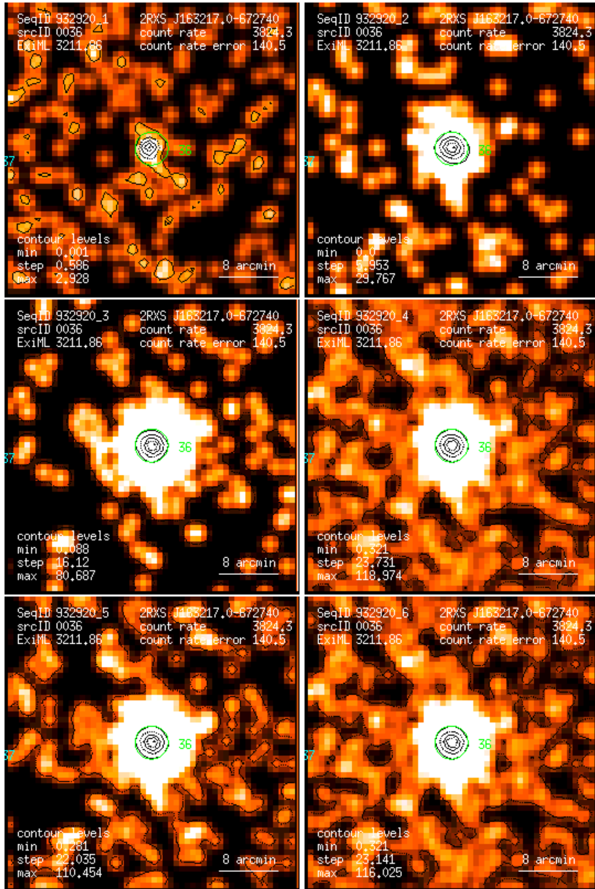
Figure 36: RASS 932920: detection 0036: band rate images, Gaussian filter: (1) PSPC channels 11 – 41, (2) 52 – 90, (3) 91 – 201, (4) 11 – 235, (5) 52 – 201, (6) 11 – 201. Broad band rates in counts/ks. Band rate contour levels in counts/ks/arcmin 2 .
